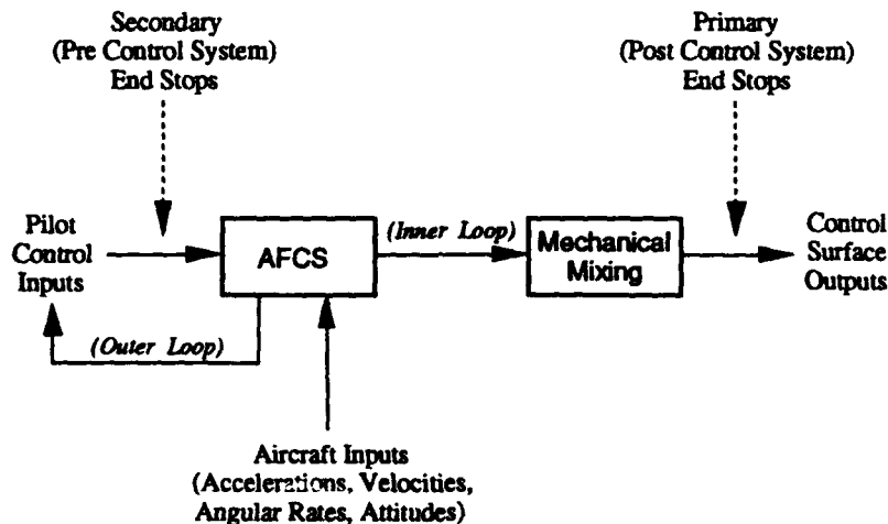
Fig. 1 Schematic Representation of Black Hawk and Seahawk Control System
