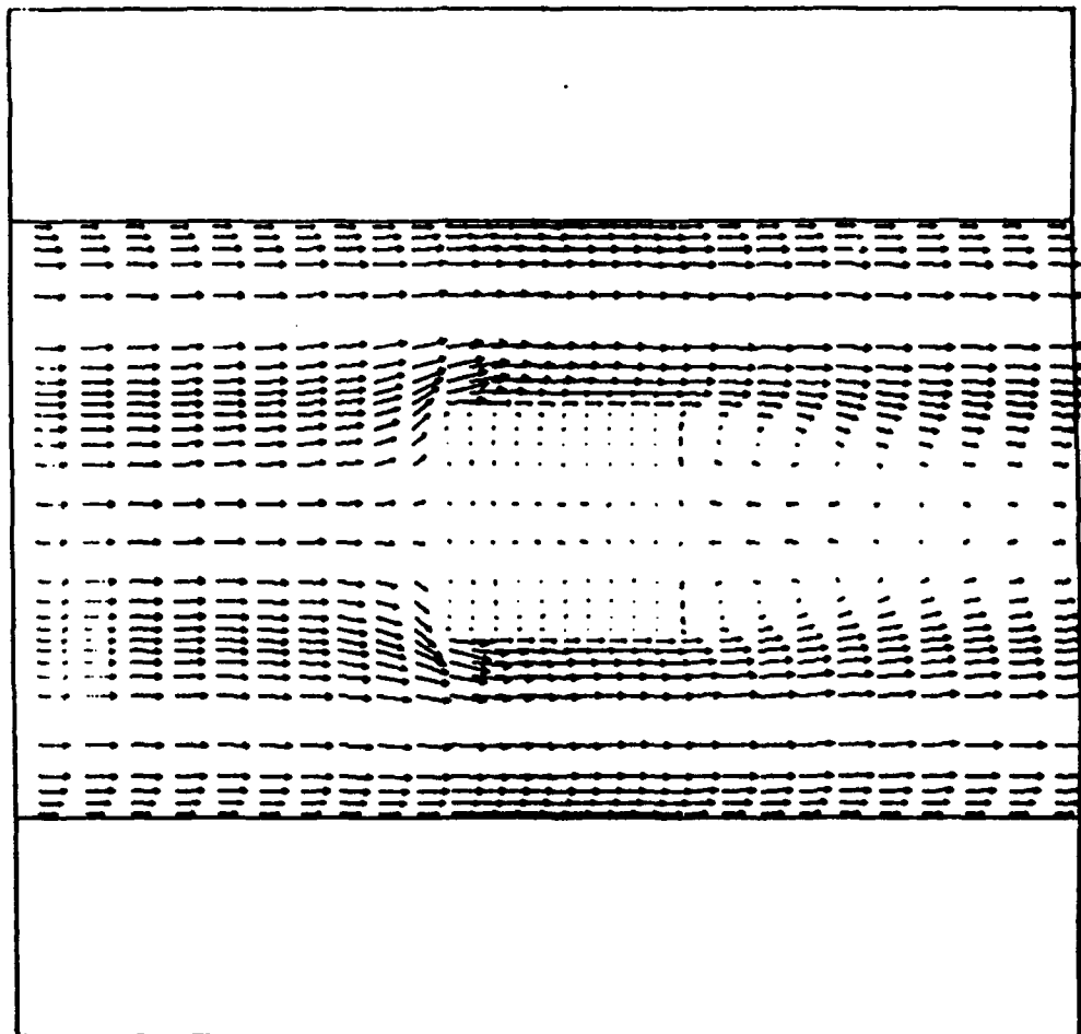
Figure 11. Velocity field for U_{\text{inlet}} = 60 \text{ in/s} and U_{\text{inject}} = 8 \text{ in/s} .
