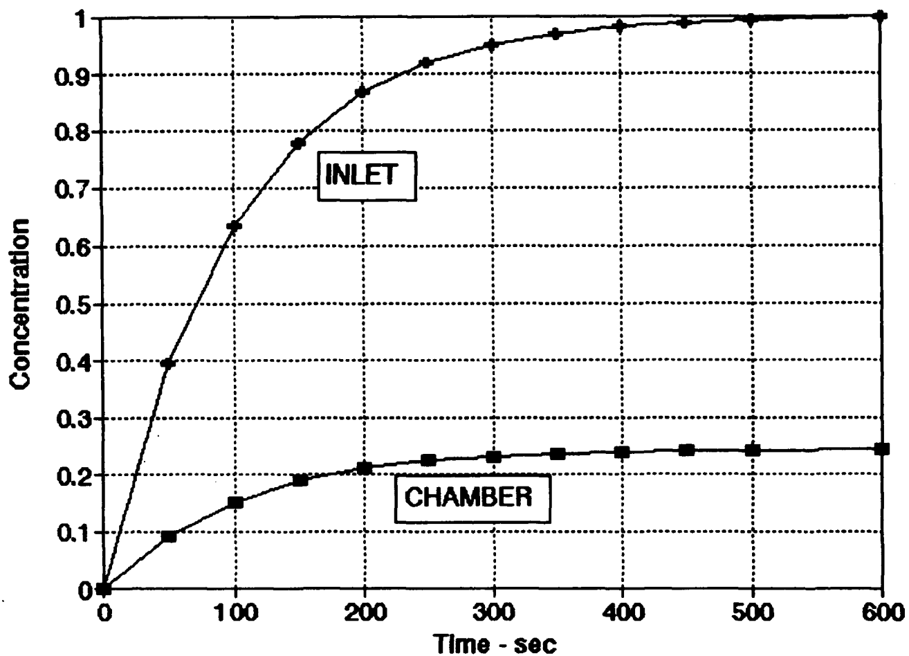
Figure 23. Transient case for U_{\text{inject}} = 16 and U_{\text{inlet}} = 60 in/s. The location in the chamber is I=64 , J=9 (1.875 in from the front of the chamber and 1.298 in from the axis).
