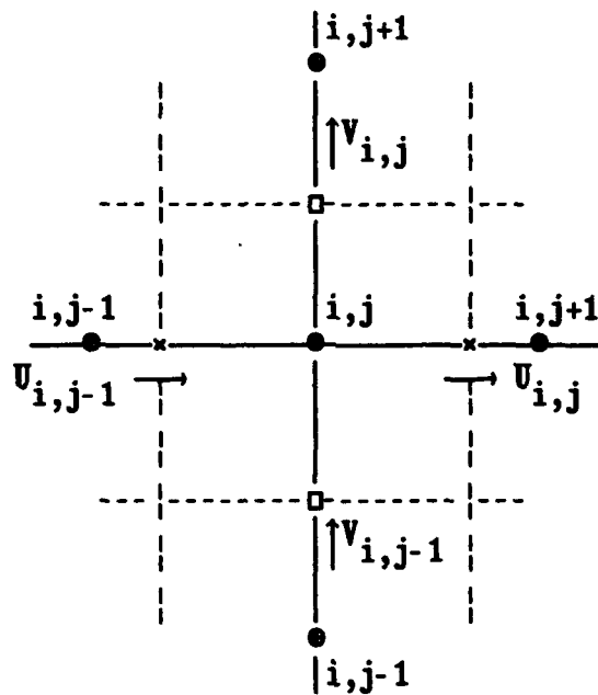
Figure 1a. The locations where u and v are evaluated, ● main grid nodes, × u-nodes, and □ v-nodes.
