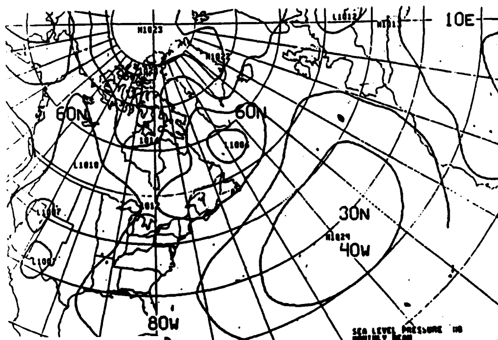
Sea level pressure (mb) Monthly mean May 1985
