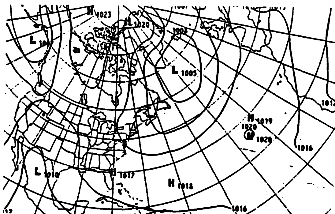
March normal sea level pressure (mb) (1948 — 1970)
