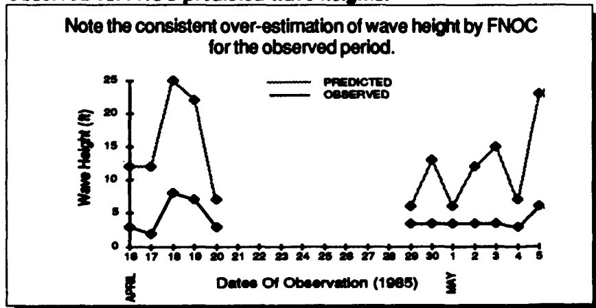
Figure C-9. Observed vs. FNOC predicted wave heights.
