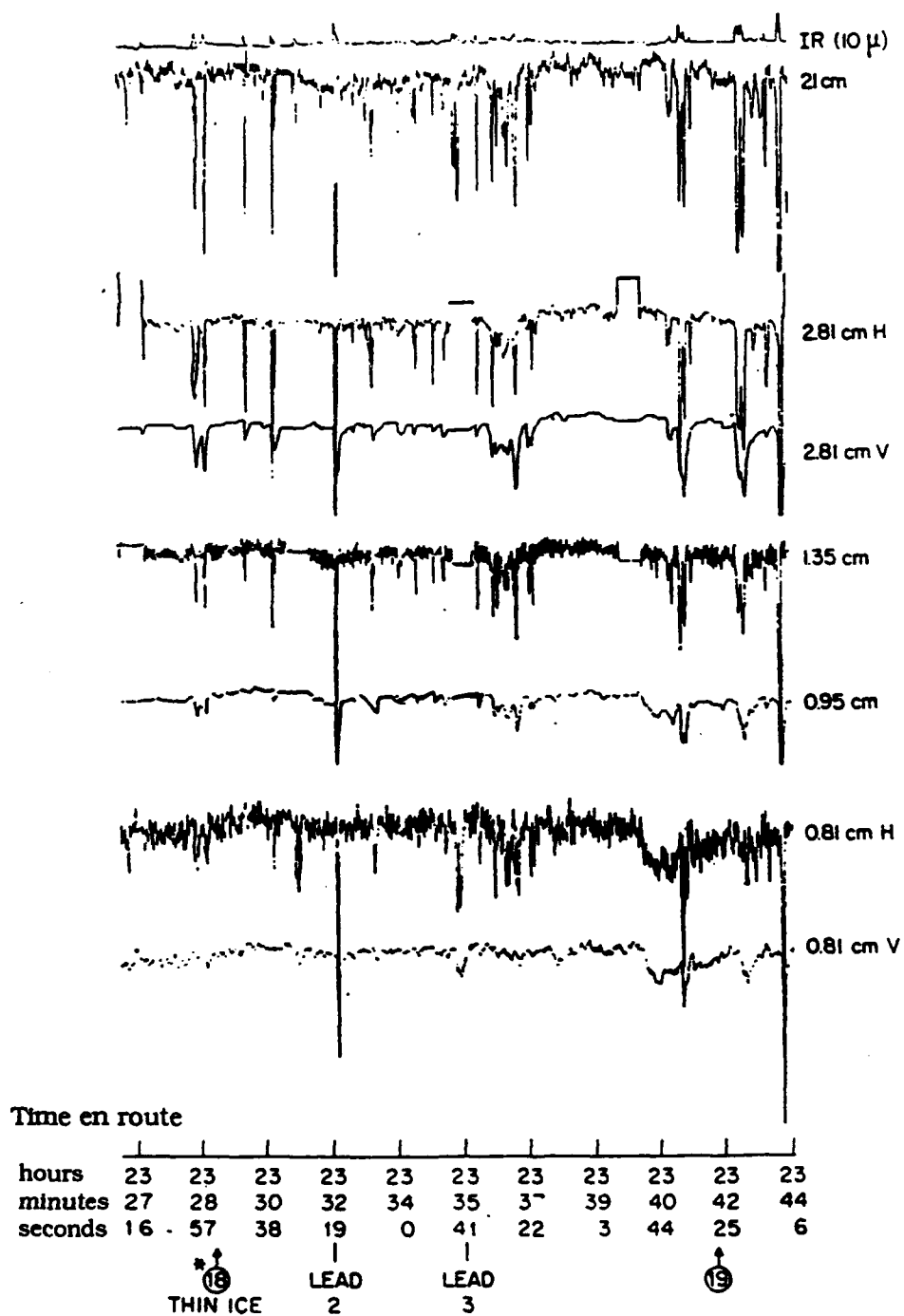
Figure 3. Multiwavelength data obtained during a low pass of the aircraft over the U.S. test area on 5 March 1973 (after Gloersen et al., 1975).
