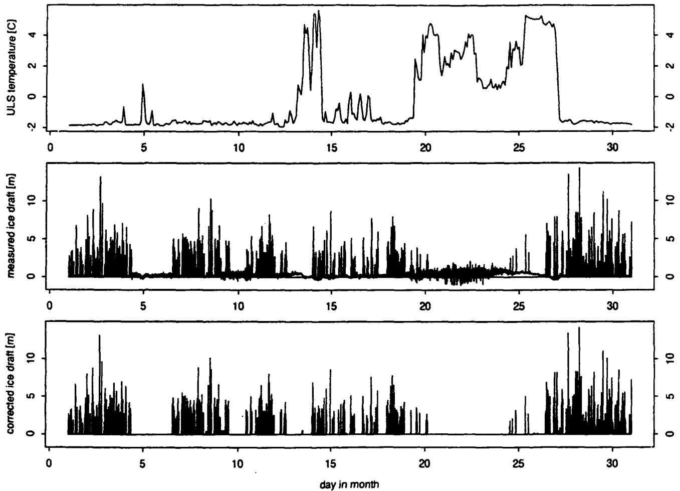
Figure 2. Temperature observations and raw and corrected ice draft recordings from the ULS at 78°N, September 1990. Note the wave effects on the recordings during the warm water influx event 18-24 September.
