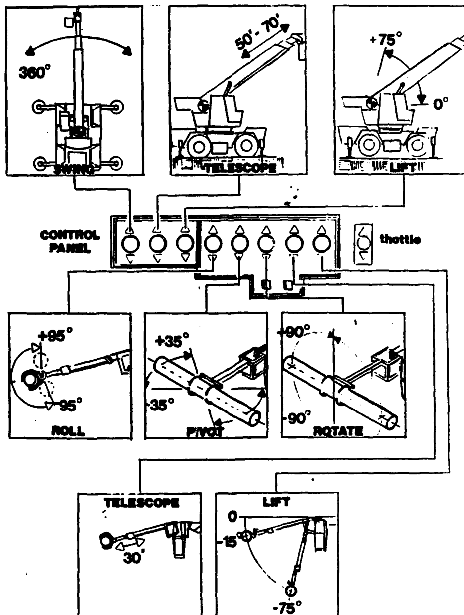
Figure 1.2: Manipulator Controls and Functions (Glass 1984)
