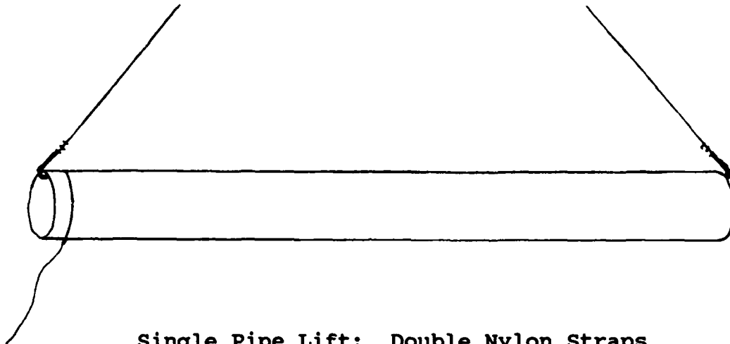
Single Pipe Lift: Double Nylon Straps
