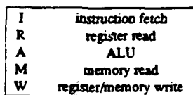
Figure 3 BAM Processor Execution Pipeline
