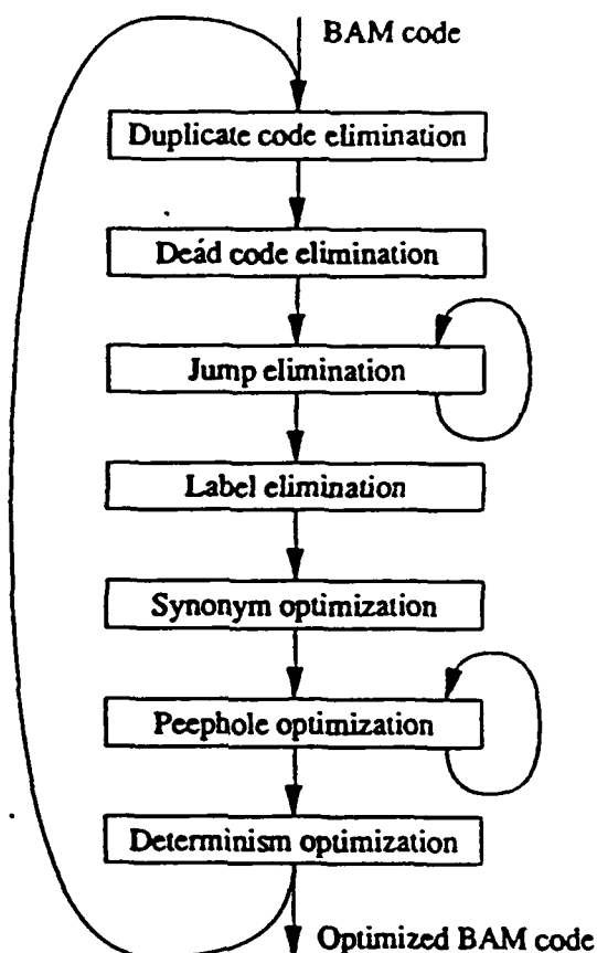
Figure 6.1 – BAM Transformations
