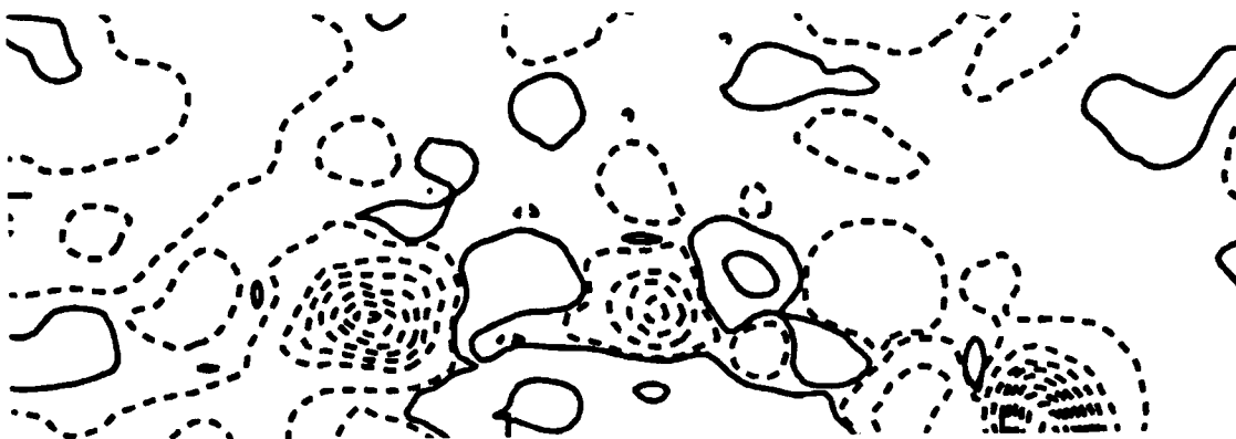
RATE-OF-STRAIN-RELATED SOURCE \left( \frac{\partial u}{\partial x} \frac{\partial v}{\partial y} \right)
