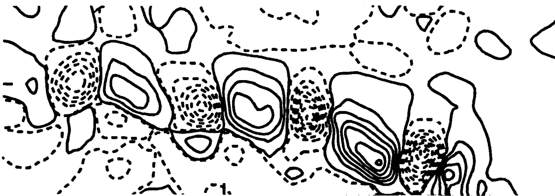
VORTICITY-RELATED SOURCE \left( \frac{\partial u}{\partial y} \frac{\partial v}{\partial x} \right)
