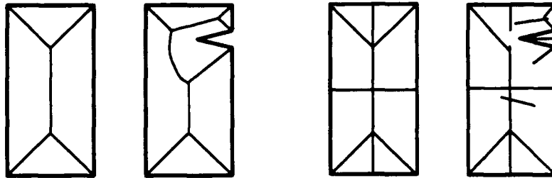
Figure 9: Skeletons found for a rectangle and a notched rectangle by SAT left and SLS right. Observe that the skeleton is highly distorted by the presence of the notch. The skeleton found by the computation presented in this paper on this shapes can be seen in Figures 7 and 8.
