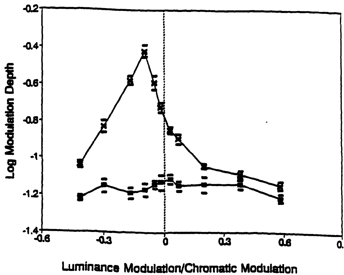
Figure 46. Empirical examples of inverted-V and flat curve. The short horizontal bars indicate \pm 1 SE.
