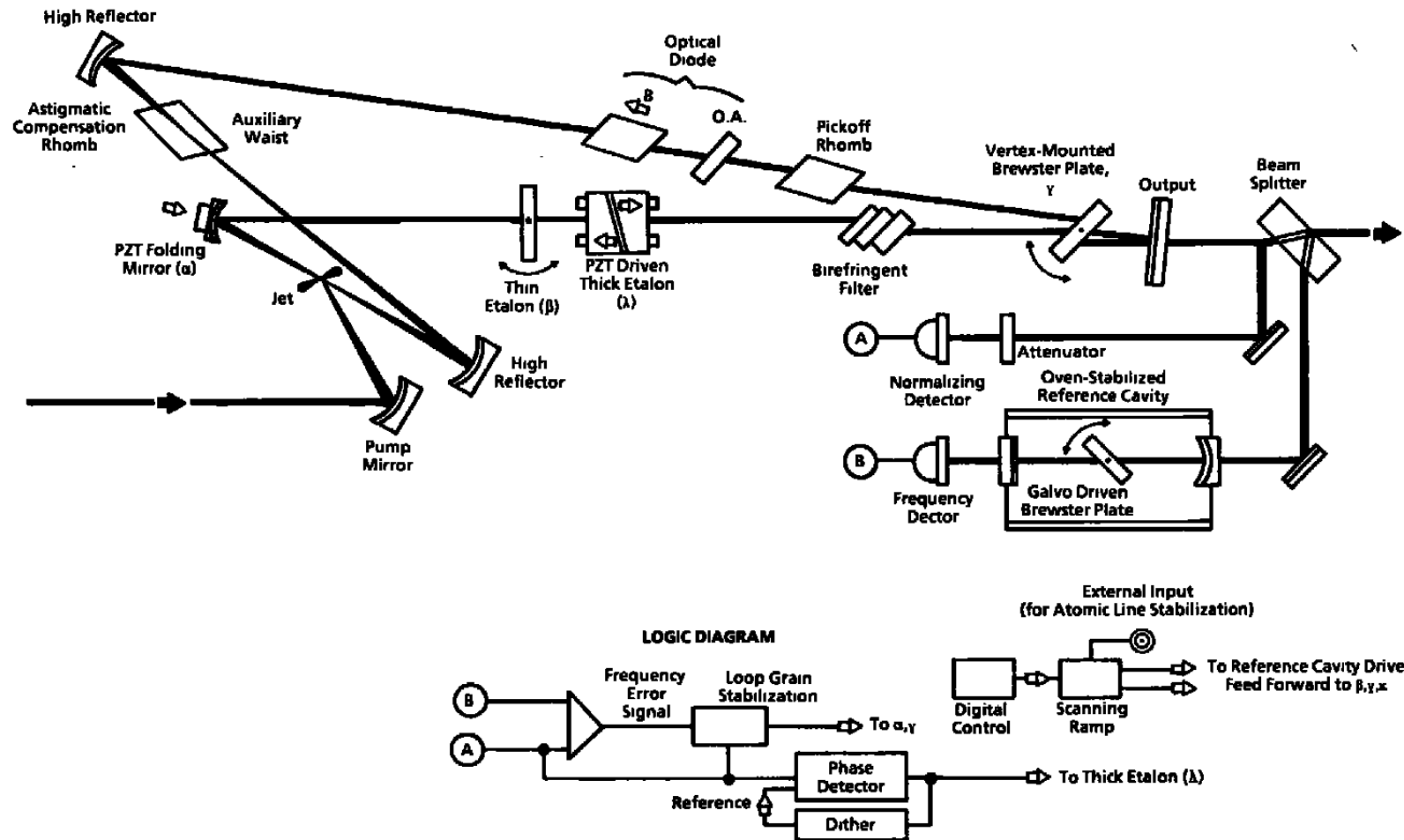
Figure 8. Ring laser cavity.
