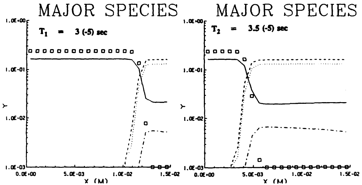
Figure 16. Major species distribution in shock tube at two time instances.
