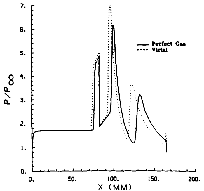
Figure 9. Comparison of projectile surface pressure distribution.
