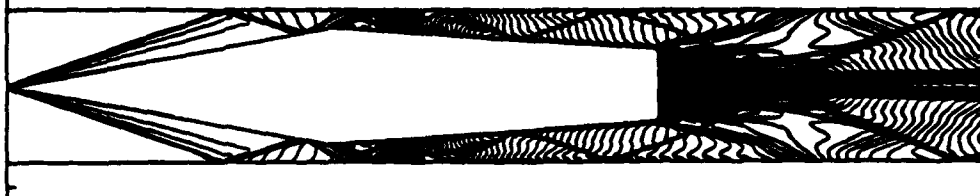
Figure 12. a) Grid obtained after multiple adaptations; b) Pressure contours on adapted grid and baseline grid; and c) Mach number contours on adapted grid and baseline grid.
