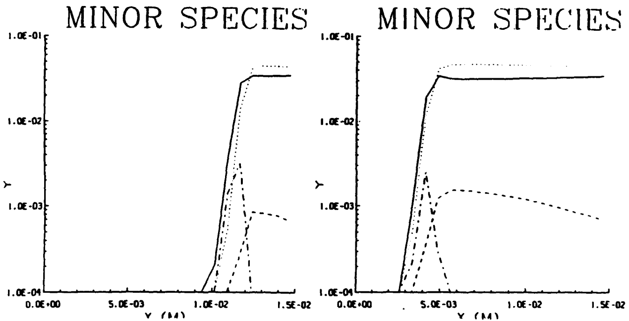
Figure 17. Minor species distribution in shock tube at two time instances.
