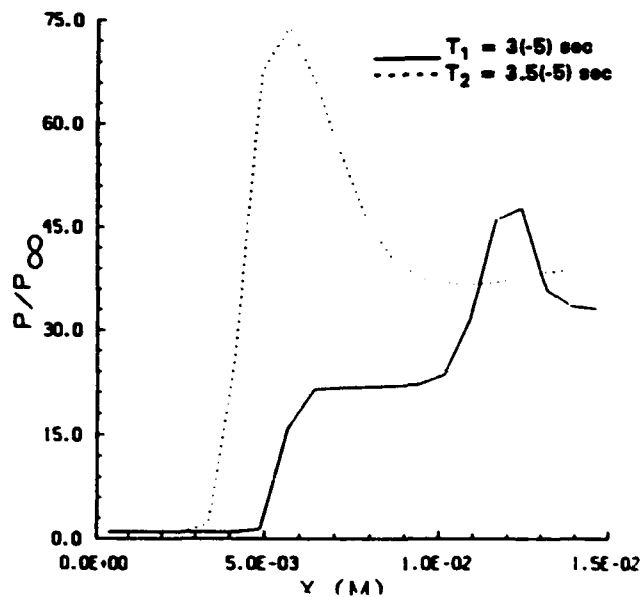
Figure 15. Pressure distribution in shock tube at two time instances.
