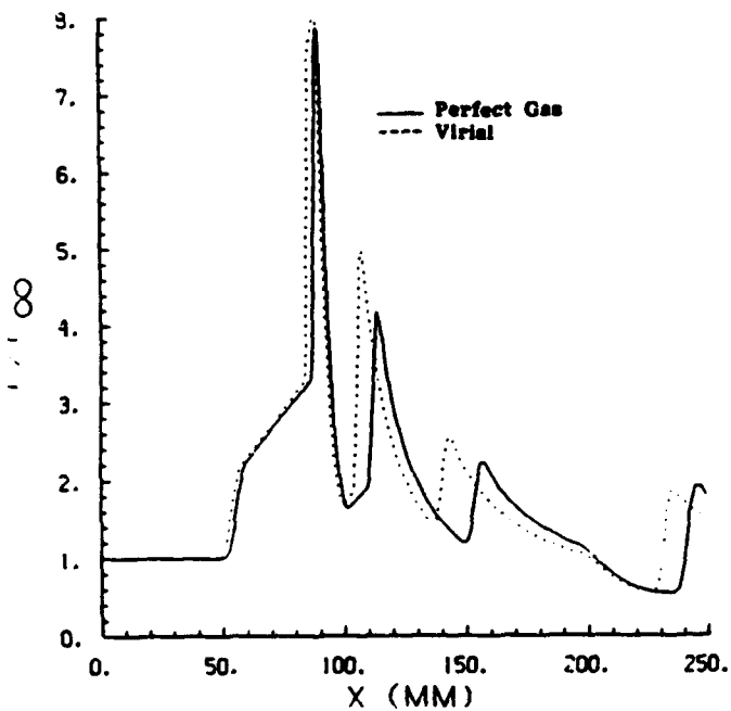
Figure 8. Comparison of tube wall pressure distribution.
