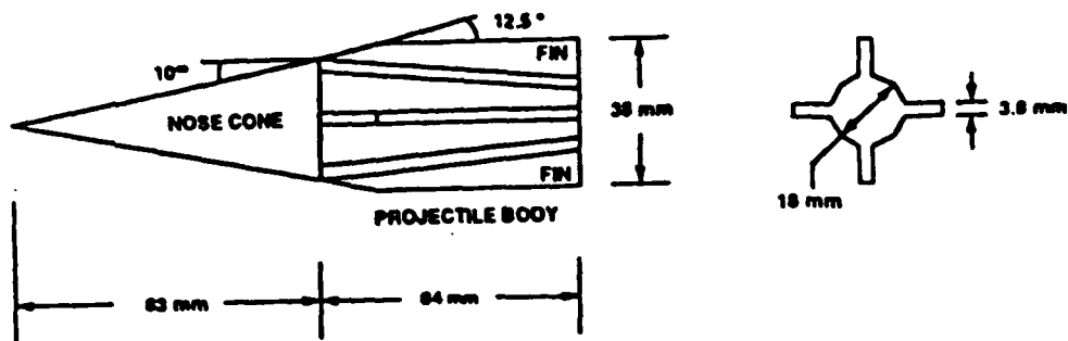
Figure 1. 38mm projectile dimensions.
