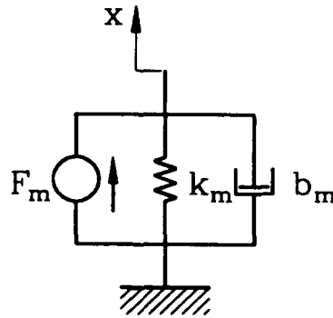
Figure 3-4. Simple model of contractile fiber.
