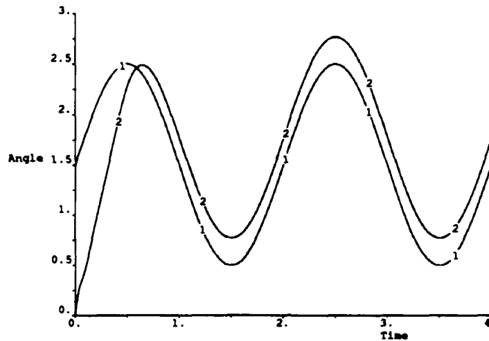
Figure 5-5. Effect of neglected joint inertia.
