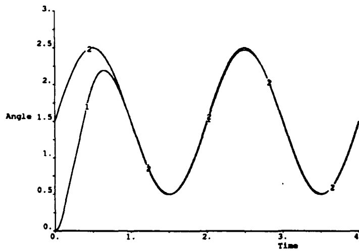
Figure 5-4. Desired and actual (modeled) joint trajectories. Zero tracking error is achieved after one second.
