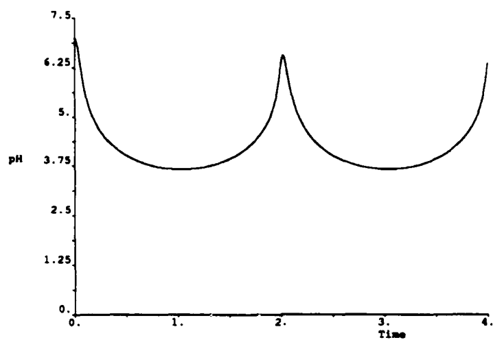
Figure 5-1. pH in the polymers fibers in response to a 1Hz input signal.
