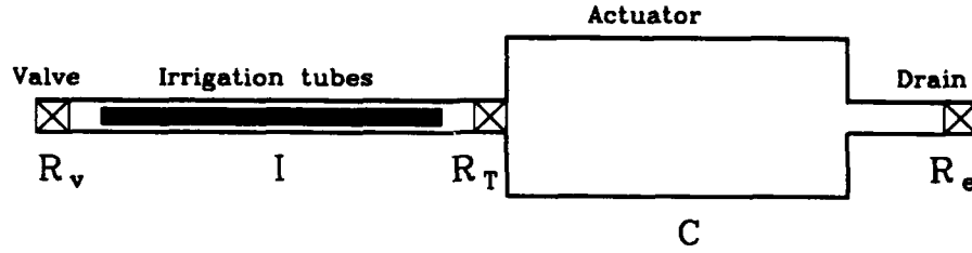
Figure 3-1. The fluid model consists of a pressure source P_0 at the inlet of the system. The valve, tubes and drain line are modeled as fluid resistances R_v , R_T and R_e respectively. Finally, a fluid inductance I is included to account for the mass of the fluid and a capacitance C to model the expansion of the actuator chamber.
