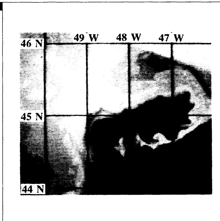
Figure C-8 Infrared image from the Advanced Very High Resolution Radiometer aboard NOAA 9 on 17 May.
