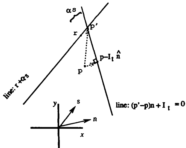
Figure 1: Two constraint lines that intersect at the corresponding point p' . The vector n is the normal component of the displacement vector, n = \nabla I and \hat{n} = \frac{\nabla I}{|\nabla I|} . The vectors n, r and the scalars \alpha, I_t are a function of the location p . The vector s is fixed for all points and can be determined only up to a scale factor.
