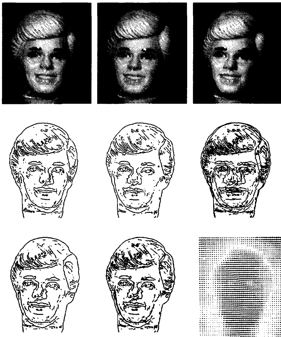
Figure 4: Results of adding flow from Ken1 to Ken4. First row: Ken1, Ken4 and the warped image Ken1-4. Second row: edges of Ken1, Ken4 and edges of both superimposed. Third row: edges of Ken1-4, edges of Ken4 and edges of Ken1-4 superimposed, flow field from Ken1 to Ken4 (scaled for display).
