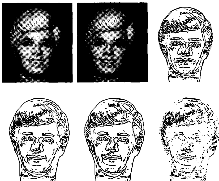
Figure 6: Comparing the four points scheme to the single privileged point scheme. First row: Ken1, Ken3 and their superimposed edge images. Second row: edges of Ken3 and Ken1-3 (the warped image) superimposed using four privileged points, edges of Ken3 and Ken1-3 superimposed using a single privileged point, the difference between edges of Ken1-3 produced by the four point scheme and the single point scheme.
