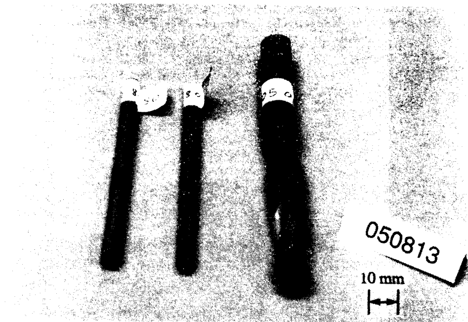
Figure 3.3-2 Photograph of three extruded CMC bits.
