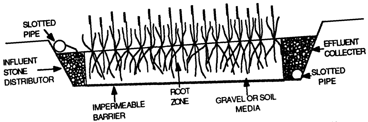
Figure II-2. Typical cross section SFCW (After EPA 1988).
