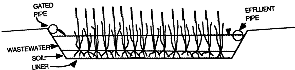
Figure II-1. Typical cross section FWS wetland.
