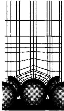
Figure 3: Side view of the high-density domain showing a 5 \times 5 \times 5 mesh along the vertical symmetry plane extending from the wall to the free stream.
