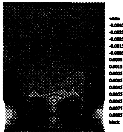
Figure 15: Cross-sectional view of the vertical velocity contours on a high-density domain with a 5 \times 5 \times 5 mesh along a vertical plane passing through the domain's inlet extending from the wall to the free stream.
