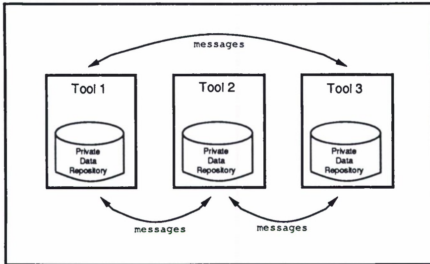
Figure 2-2 Integration Through Message Passing
