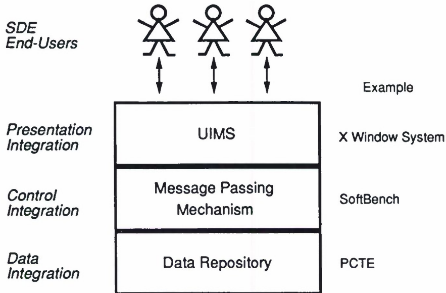
Figure 5-2 A Possible SDE Architecture?
