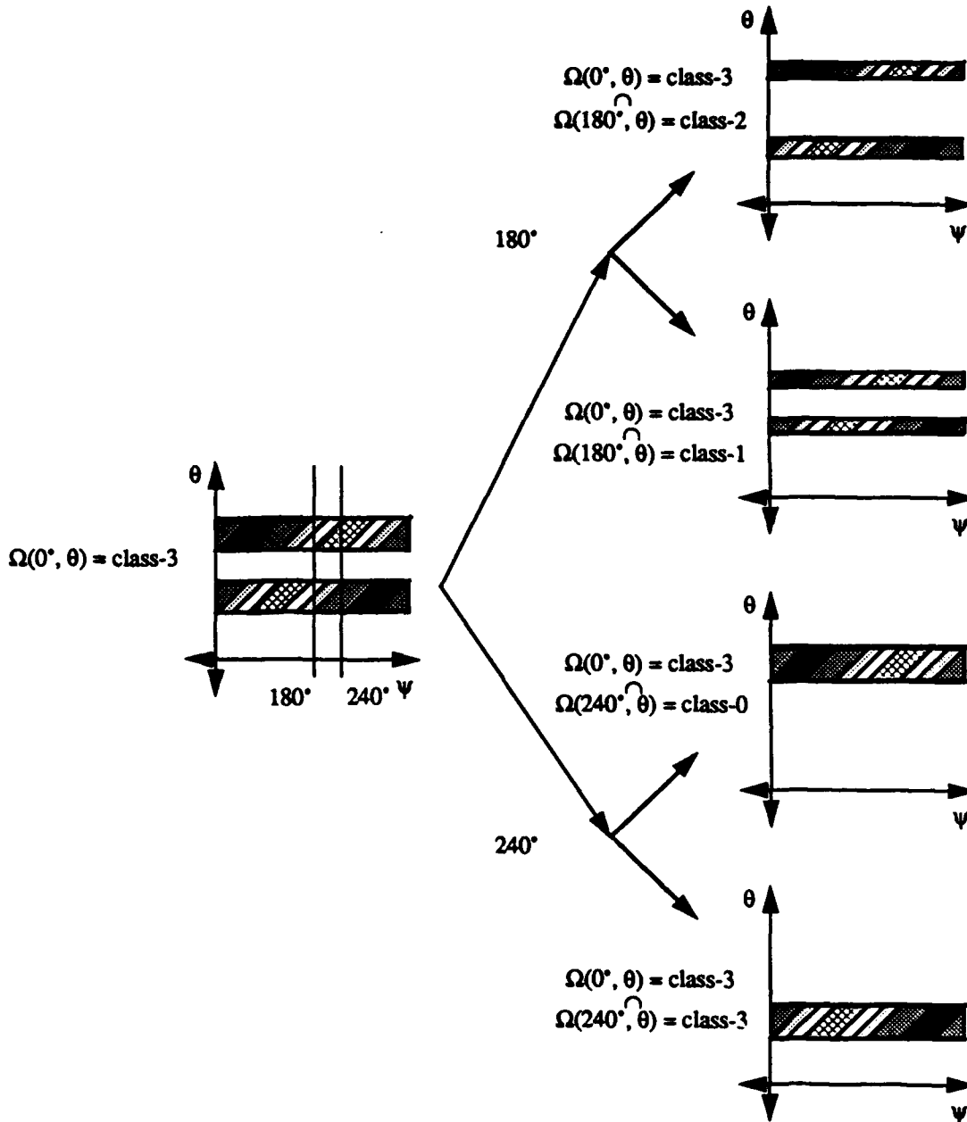
Figure 10: Two Possible Moves Following \Omega(0^\circ, \theta) = \text{class-3}
