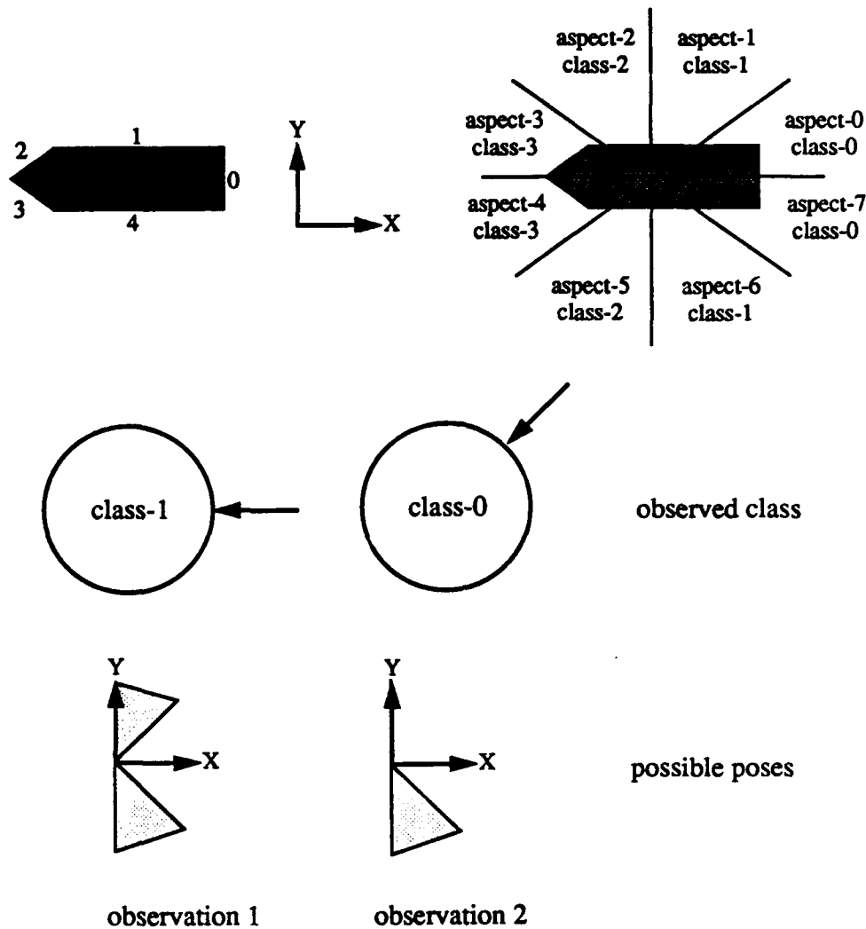
Figure 3: Resolution of Congruent Aspects
