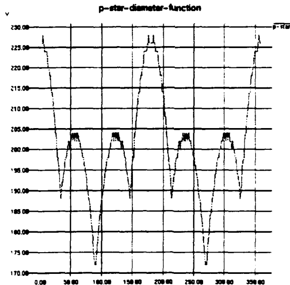
Figure 25: Sampled Diameter Function for Planar Object p-star
