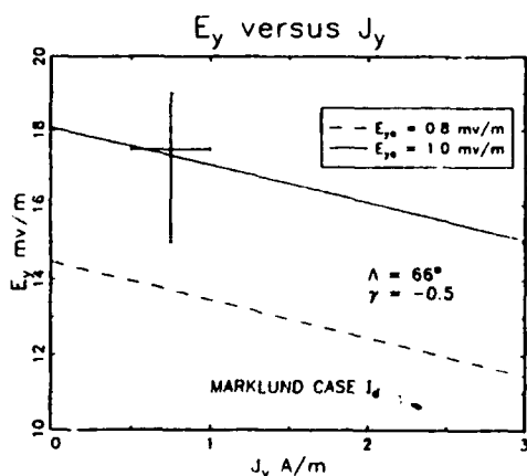
Fig. 5. The east west electric field E_y inside the auroral arc as predicted by the model. Note that the 1.0 mV/m value for E_{ye} gives better agreement as is the case in Figure 4.
