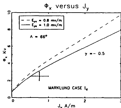
Fig. 4. Comparison of the field-aligned potential drop along the poleward boundary \Phi_x as a function of the diverted current J_y . It is seen that a 1.0 mV/m cross-tail electric field E_{ye} gives better agreement.
