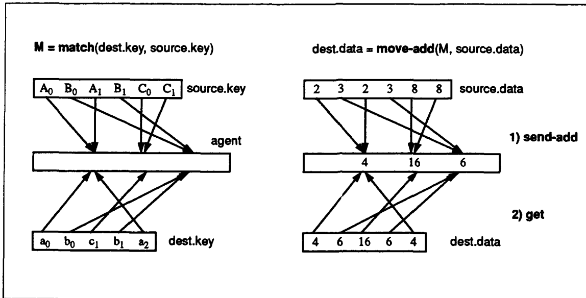
Figure 9.7: A mapping may be created by using parallel hashing. The mapping data structure directs all equal keys to the same agent site. A move operation is executed by combining source values in the agent, and then retrieving copies for each destination.
