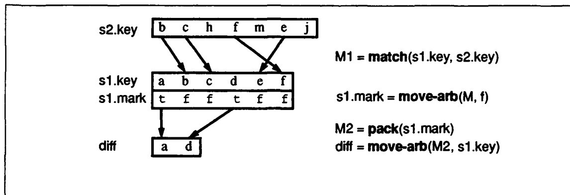
Figure 5.6: Set Difference. Marks are used to indicate elements in one set that are not in the other. Unmarked elements are then removed by using a packing step.
