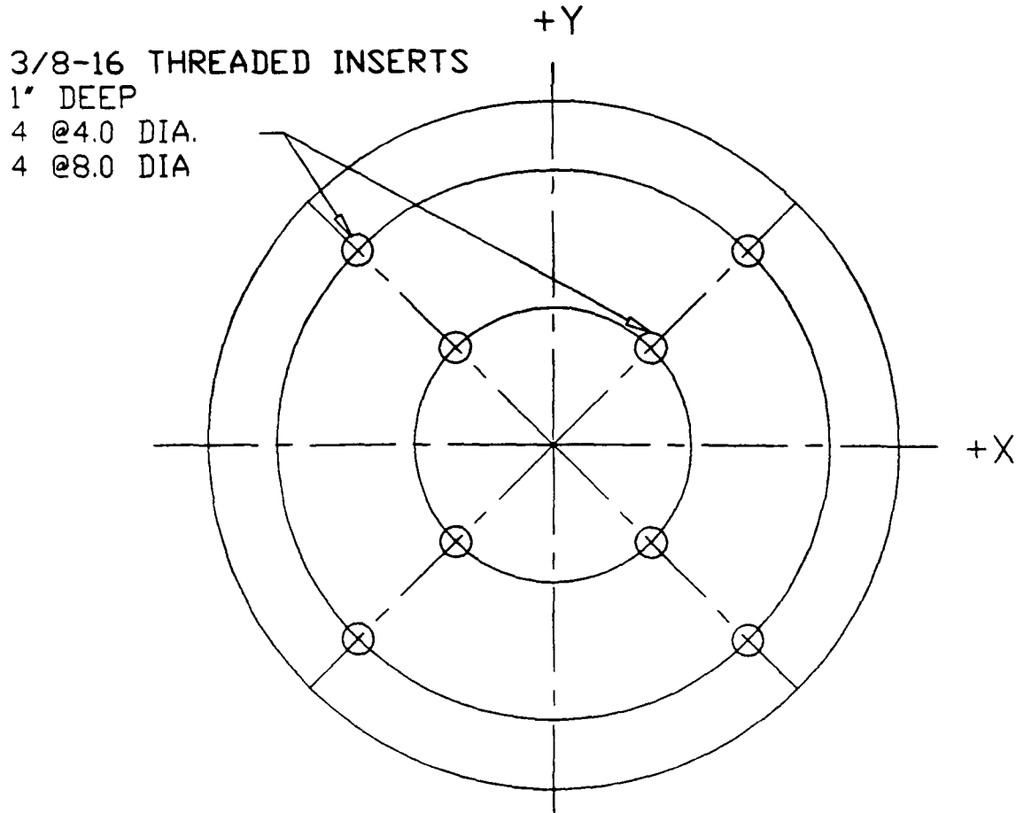
Figure D-1. Mounting pattern of test platform.
