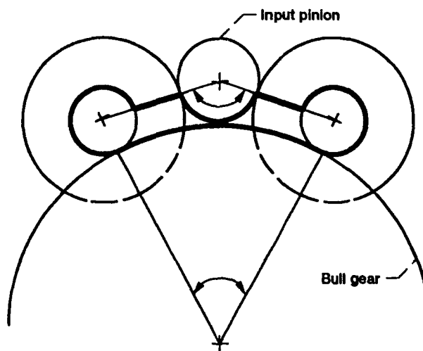
Figure 1.—Split-torque geometry.
