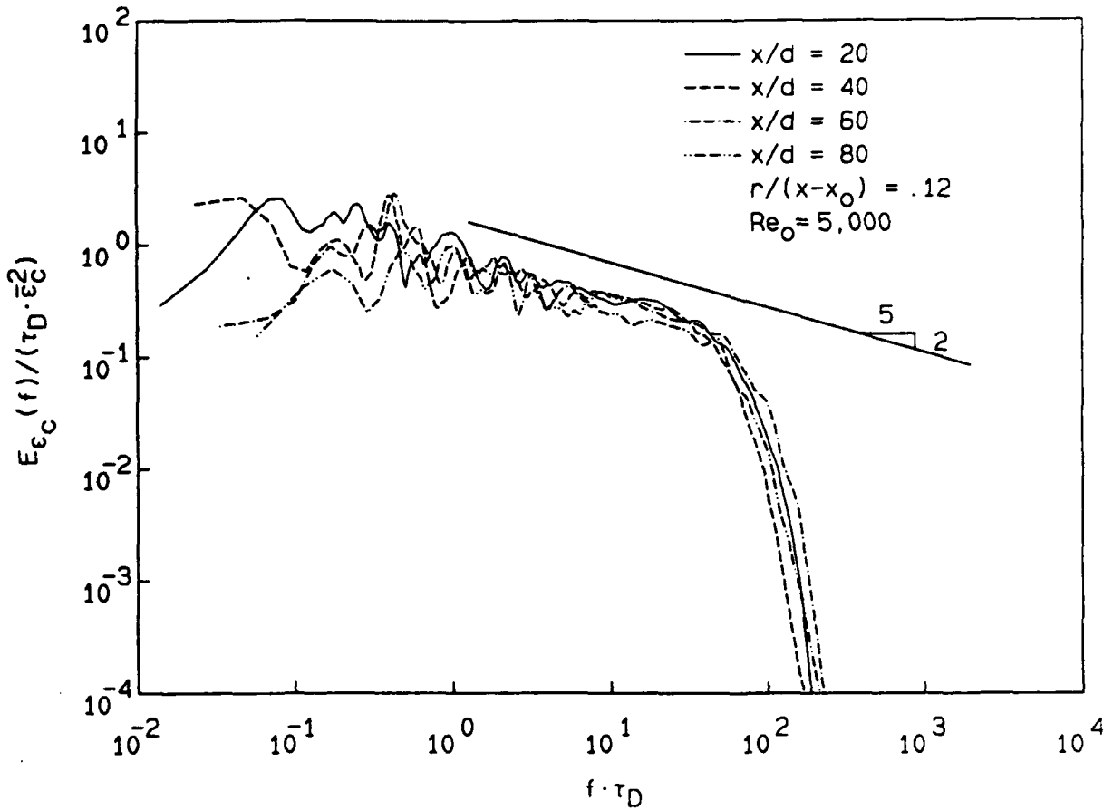
Figure 7-7. Power spectra of \epsilon_c 7^0 off the centerline at Re_0 = 5,000 .
