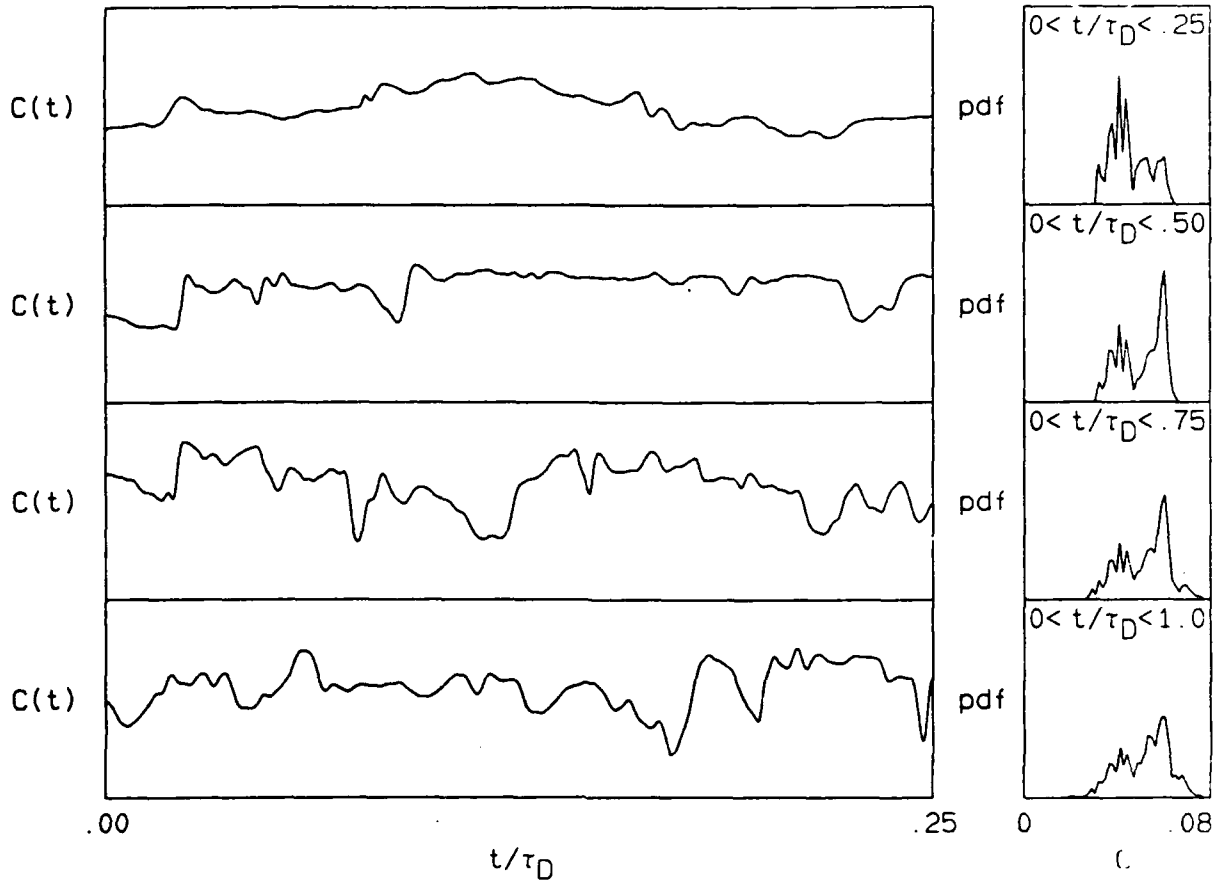
Figure 5-11. Time traces of C(t) and accumulated PDFs at Re_0 = 16,000 on the jet centerline with about .25 \tau_D per line.
