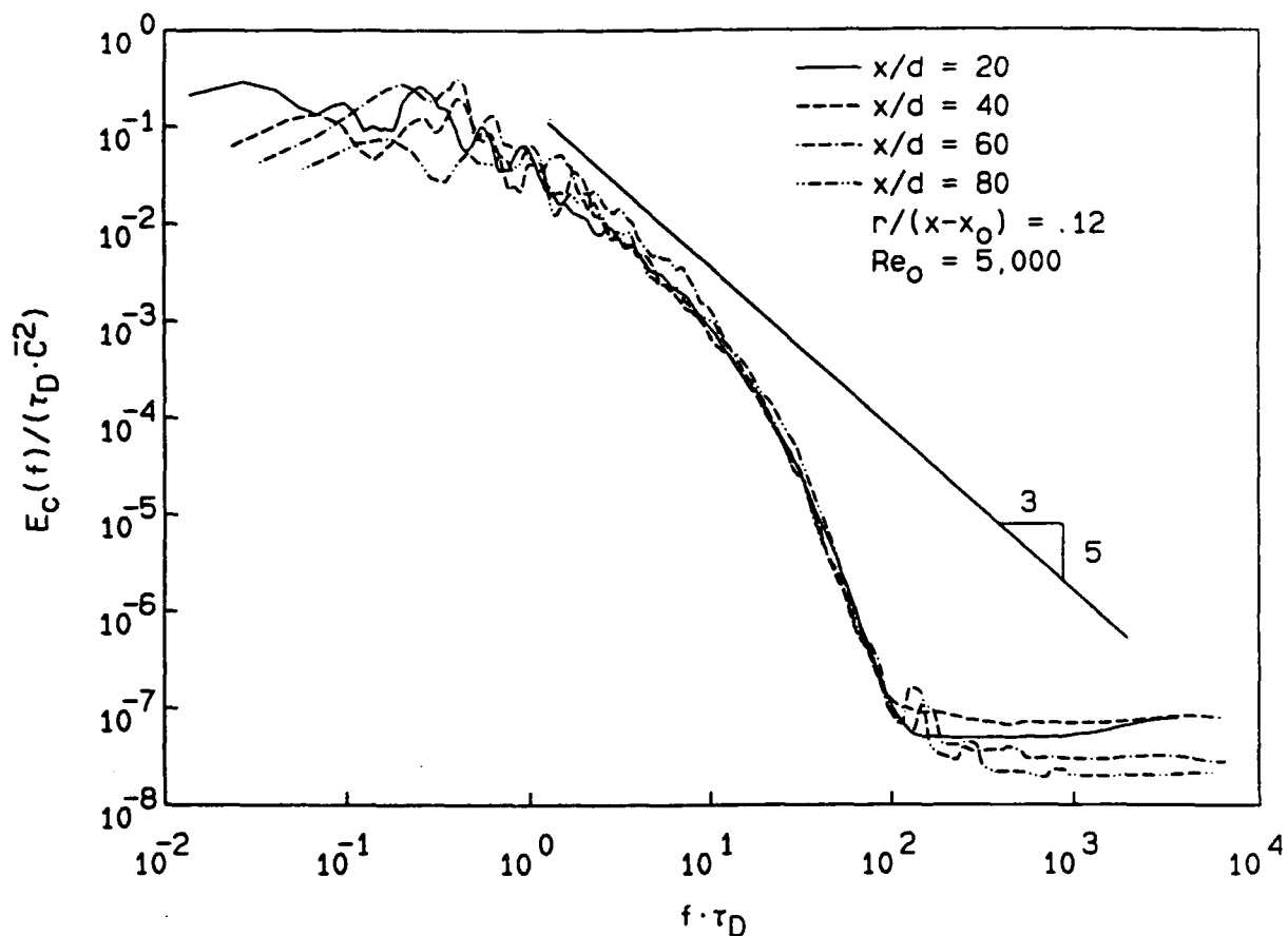
Figure 4-3. Scaled power spectra of the concentration fluctuations 7^\circ off the jet centerline at Re_0 = 5,000 .
