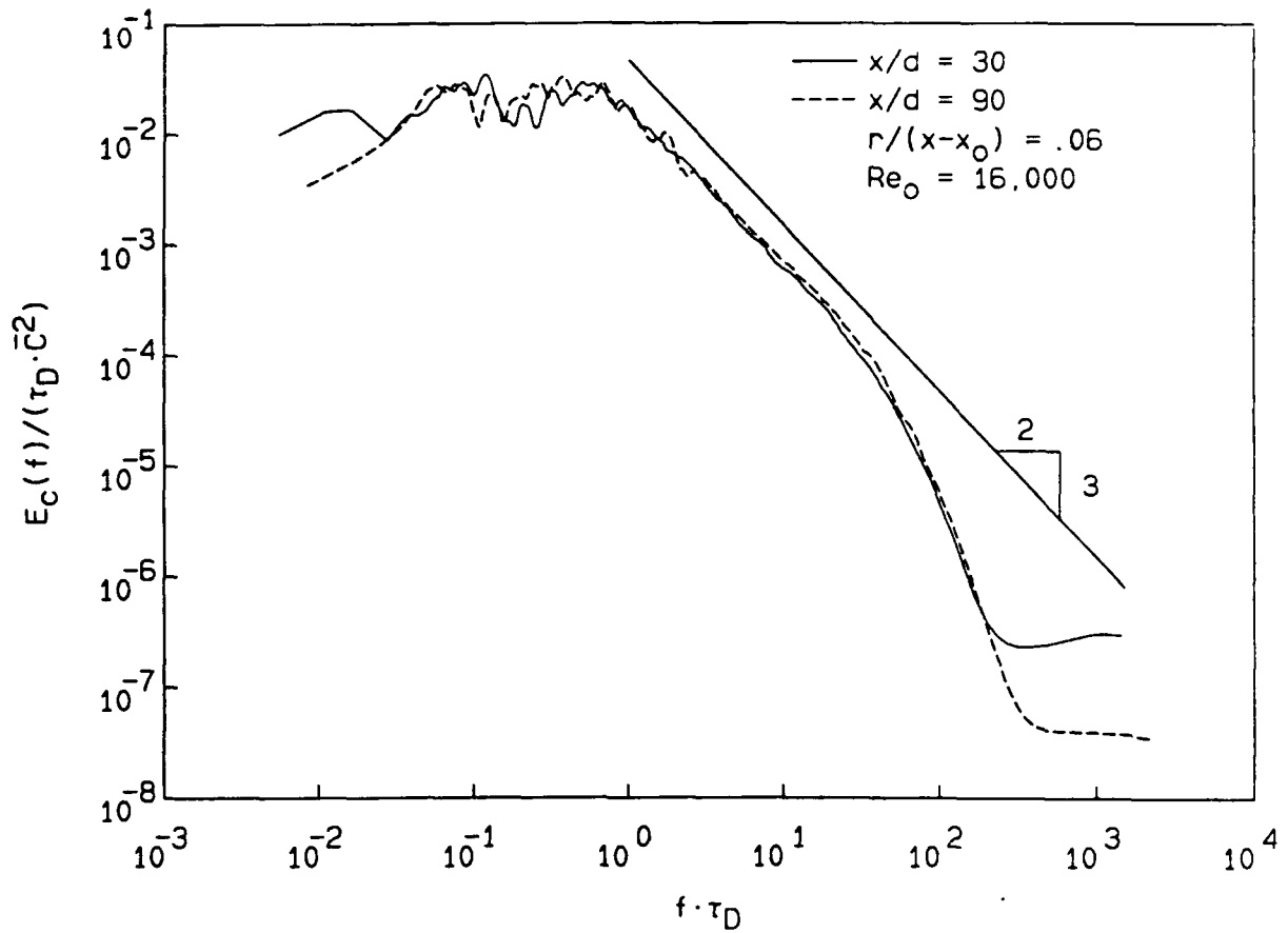
Figure 4-5. Scaled power spectra of the concentration fluctuations 3.4^\circ off the jet centerline at Re_0 = 16,000 .
