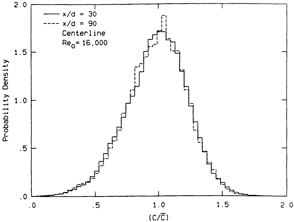
Figure 5-4. Probability density function of the scaled concentration on the jet centerline at Re_0 = 16,000 .
