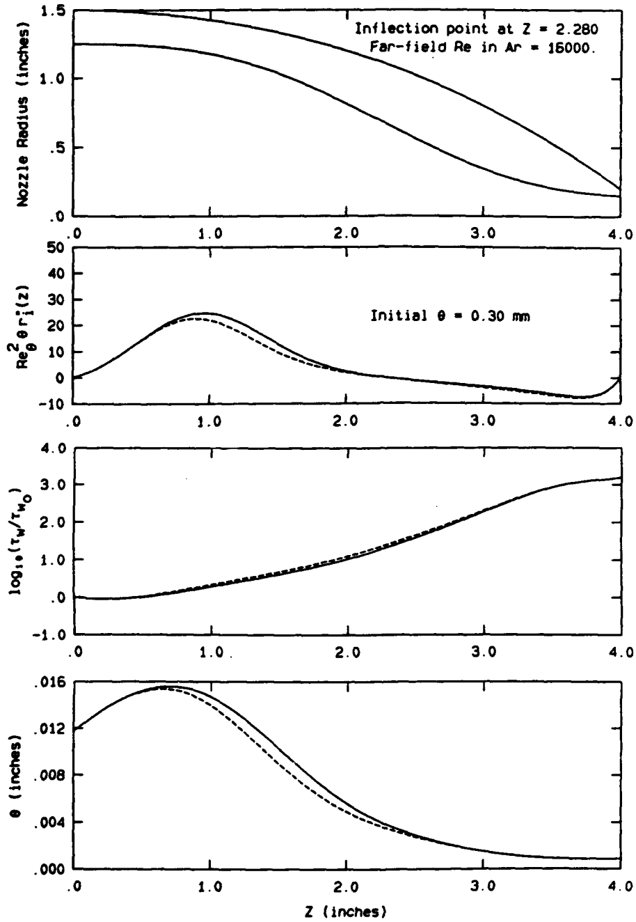
Figure A-2. Results of the design analysis for the 0.30" nozzle.
