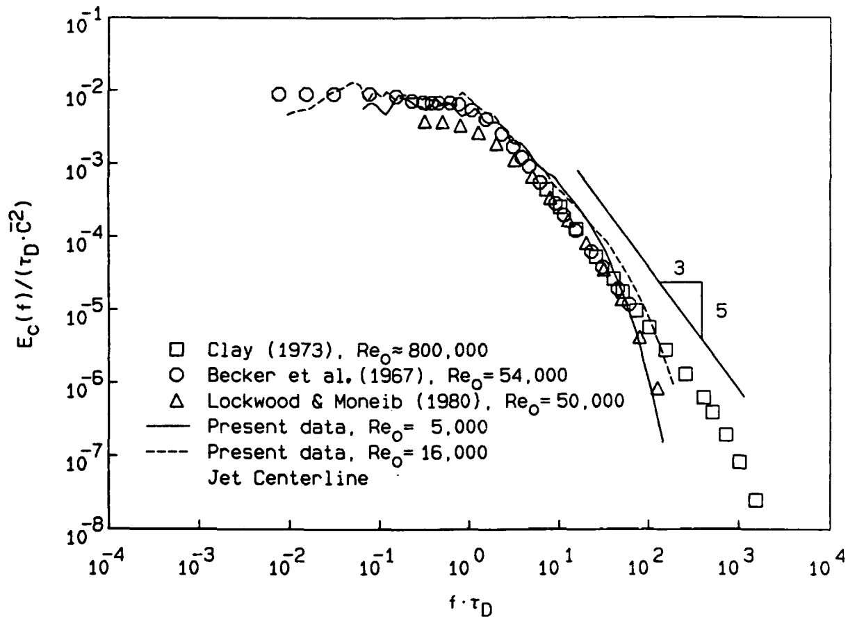
Figure 4-7. Comparison of the centerline concentration fluctuation power spectra to the results of other experiments with jet parameter scaling of the axes.
