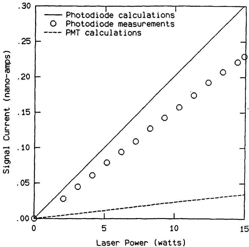
Figure B-1. Linearity of the photodetectors.
