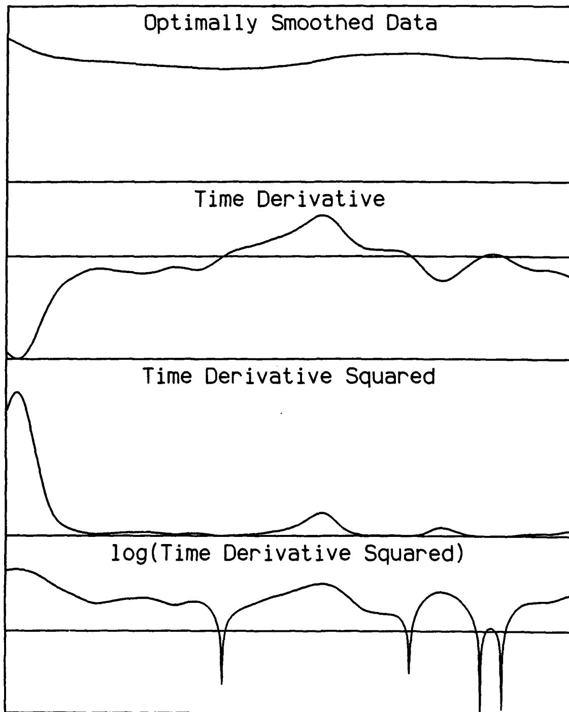
Figure E-4. Effects on the optimally filtered concentration of taking the time derivative, squaring the time derivative, and taking the logarithm of the square of the time derivative.
