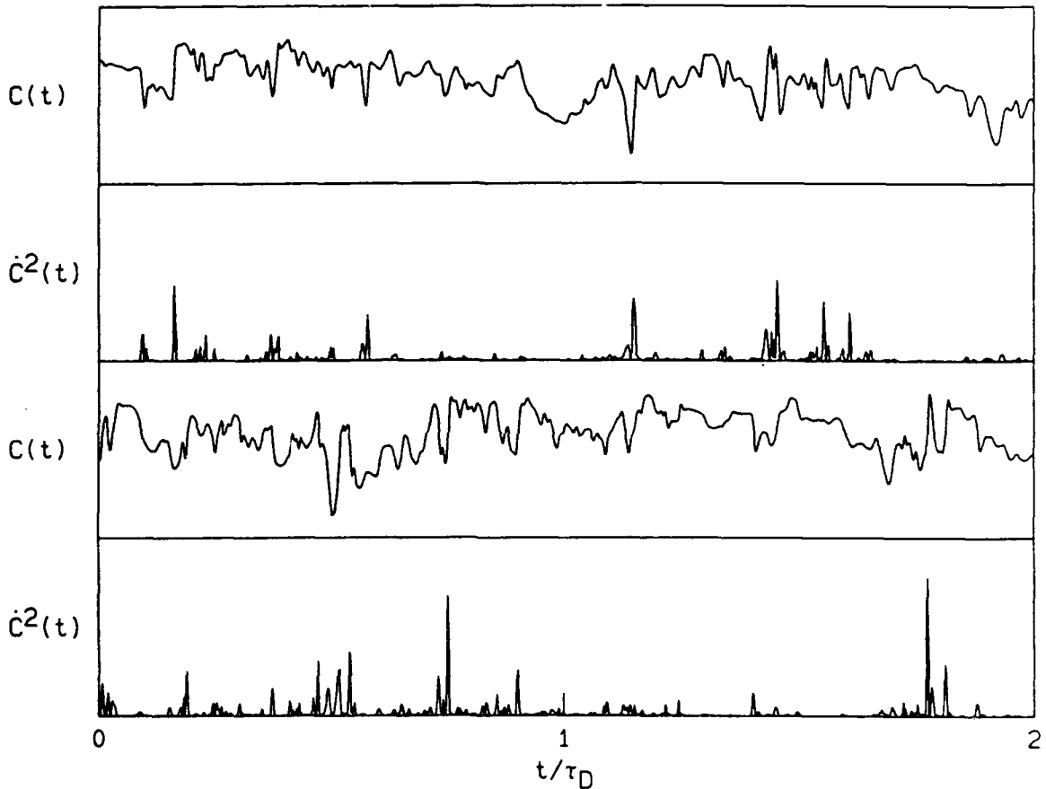
Figure 7-2. Time traces of C(t) and \epsilon_c(t) on the jet centerline at Re_0 = 5,000 .
