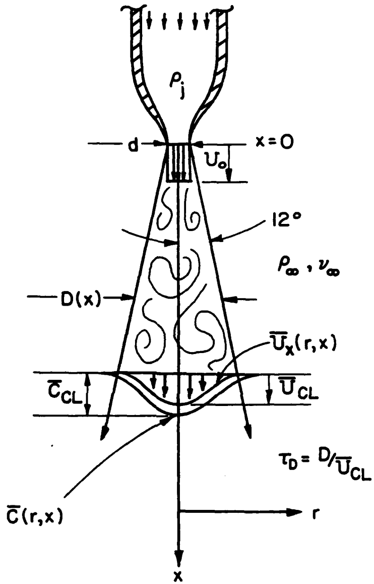
Experimental Jet Flow Coordinates
