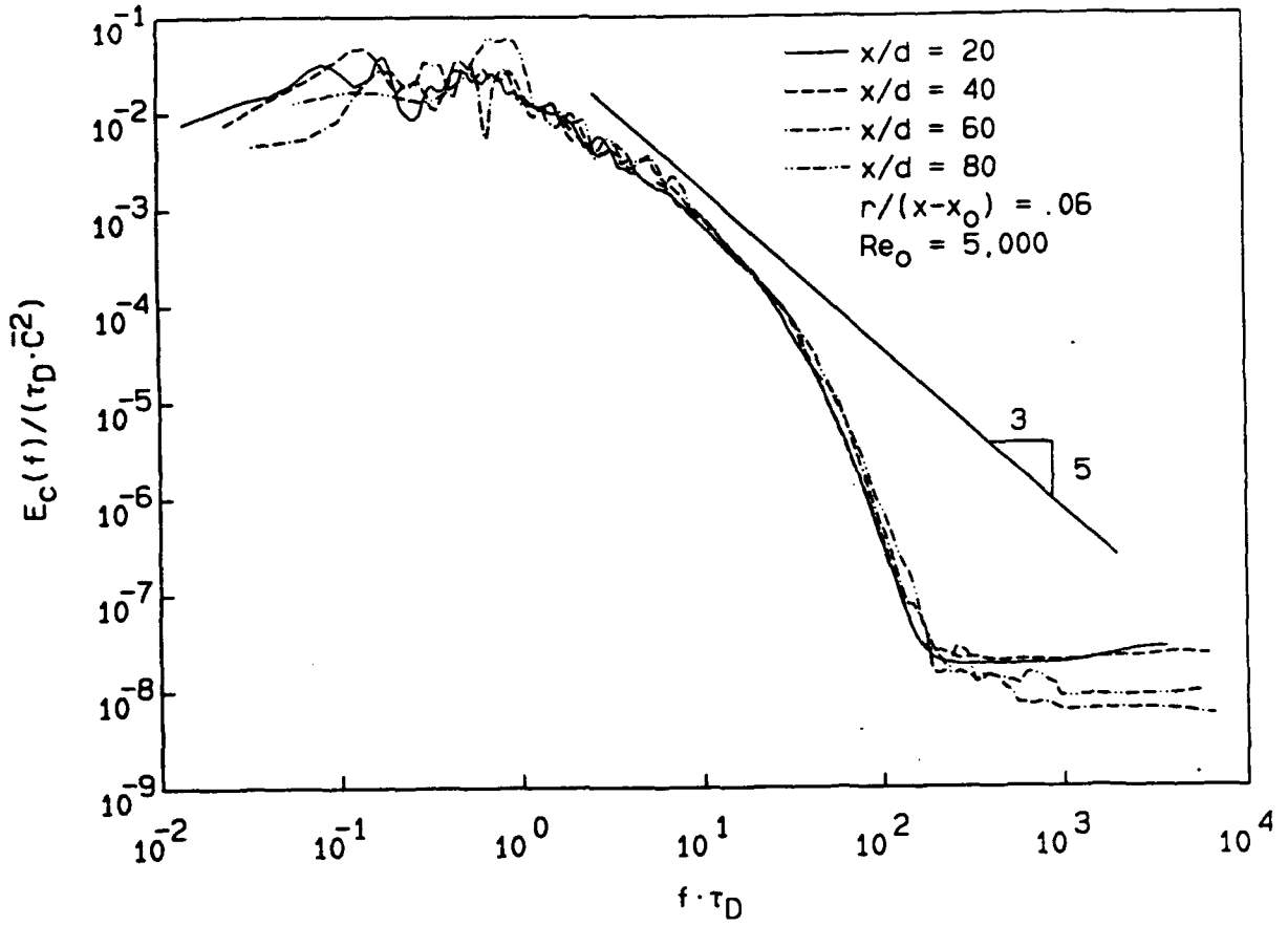
Figure 4-2. Scaled power spectra of the concentration fluctuations 3.4^\circ off the jet centerline at Re_0 = 5,000 .
