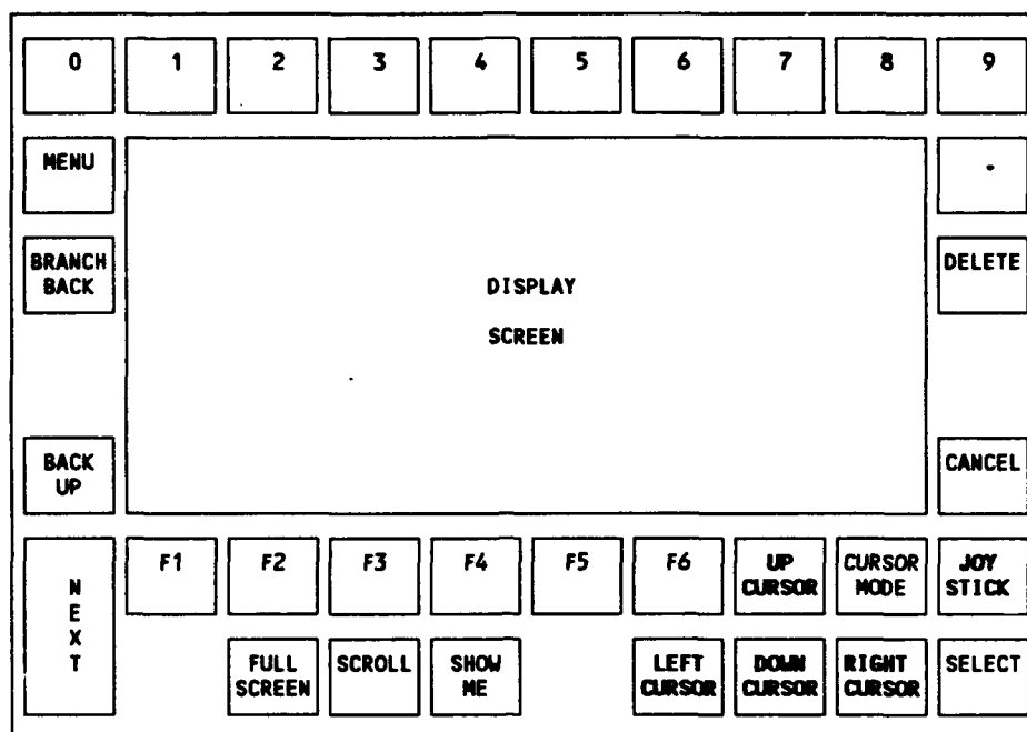
Figure 4. IMIS Portable Maintenance Aid (PMA) Layout
