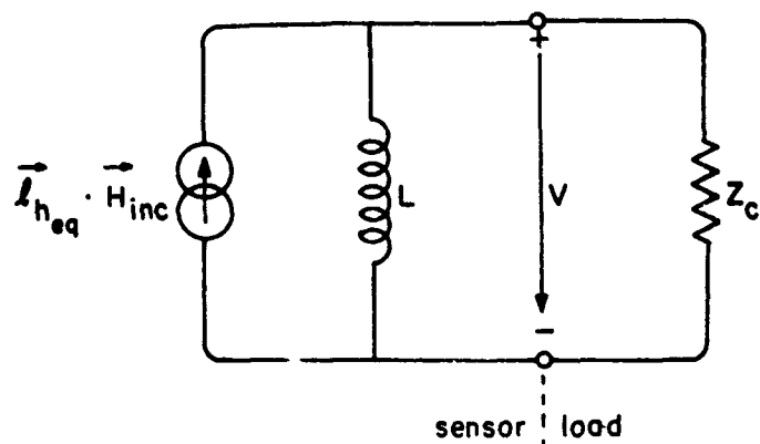
B. Norton equivalent circuit
