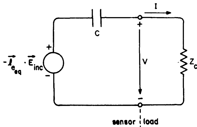
A. Thevenin equivalent circuit
