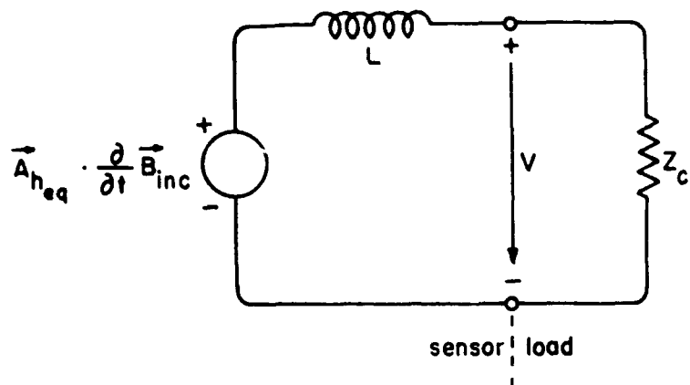
A. Thevenin equivalent circuit
