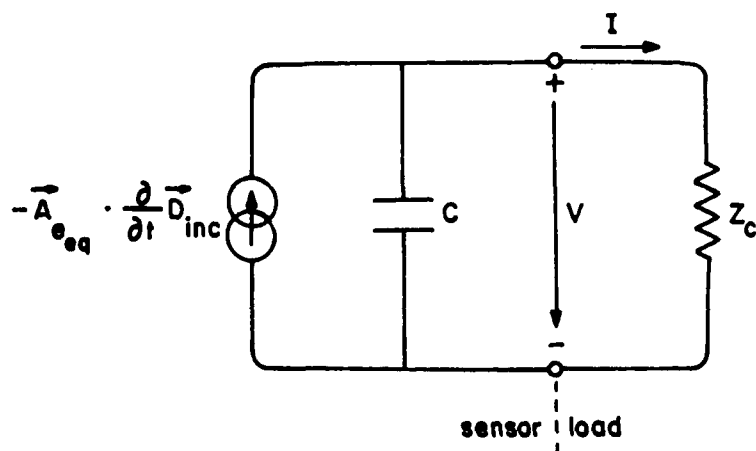
B. Norton equivalent circuit
