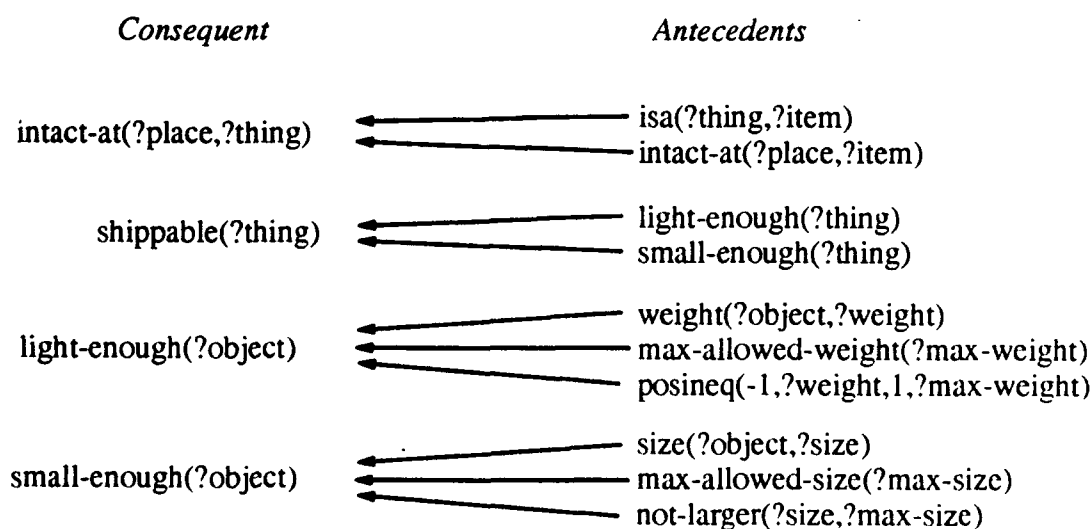
Figure 3.3. Inference Units for the Package-Sending Domain
