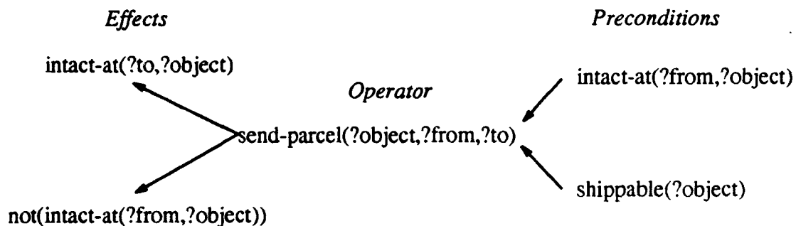
Figure 3.2. An Operator Unit
