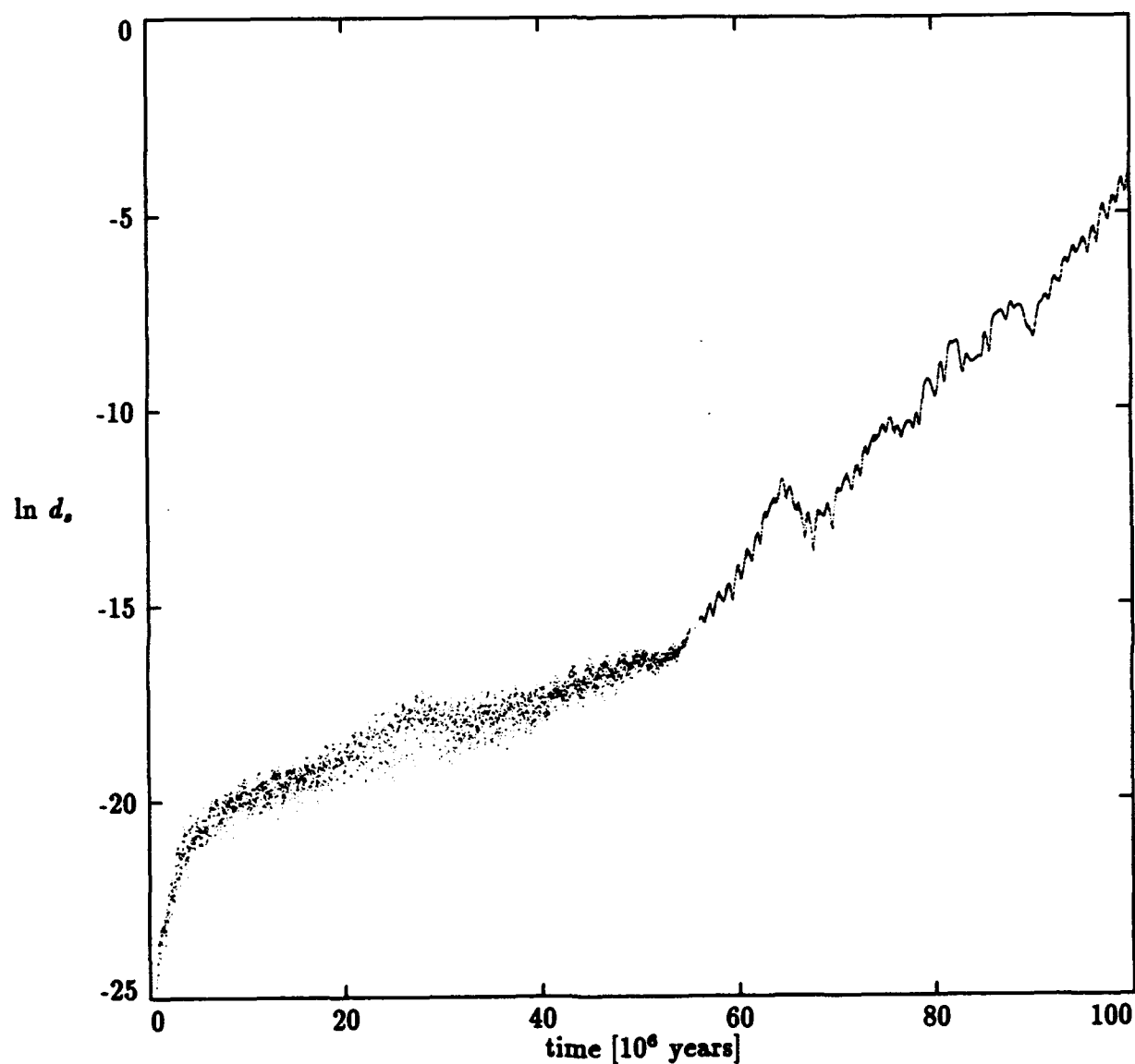
Figure 1: Exponential divergence of nearby trajectories is indicated by the average linear growth of the logarithm of the full secular phase space distance between two different runs with very slight differences in initial conditions. The segment following the initial transient has an exponential timescale of about 12 million years. The divergence is subsequently dominated by an exponential with a timescale near 4 million years.
