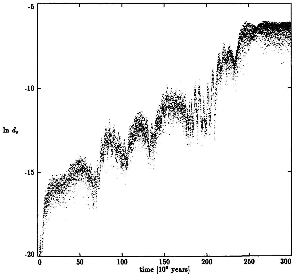
Figure 5: The secular phase space divergence of the trajectories of Jupiter in the 28 day Stormer integrations show a timescale for exponential divergence that is somewhat longer than 20 million years. The divergence saturates after about 250 million years at a rather small value, perhaps indicating a hidden constraint on the trajectories.
