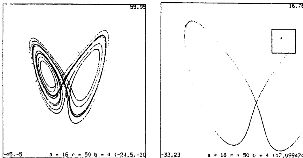
Figure 7: Lorenz Attractor for a = 16 , r = 50 and b = 4
