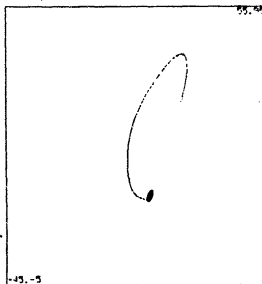
Figure 11: Segmented Path to a Fixed Point
