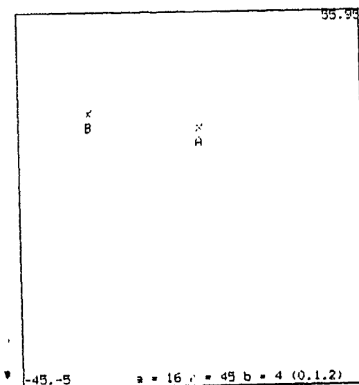
Figure 3: Origin and Destination Points
