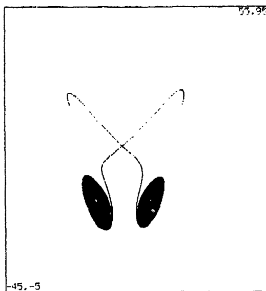
Figure 4: Two Stable Fixed Points
