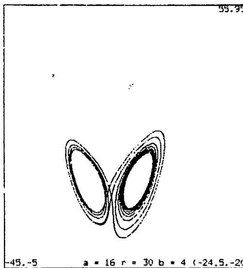
Figure 5: Lorenz Attractor for a = 16 , r = 30 and b = 4
