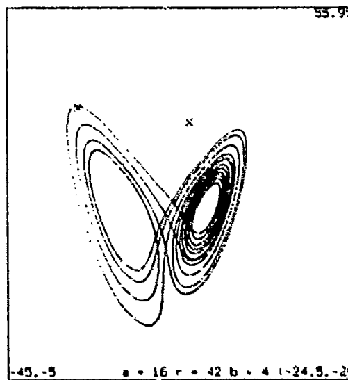
Figure 6: Lorenz Attractor for a = 16 , r = 42 and b = 4
