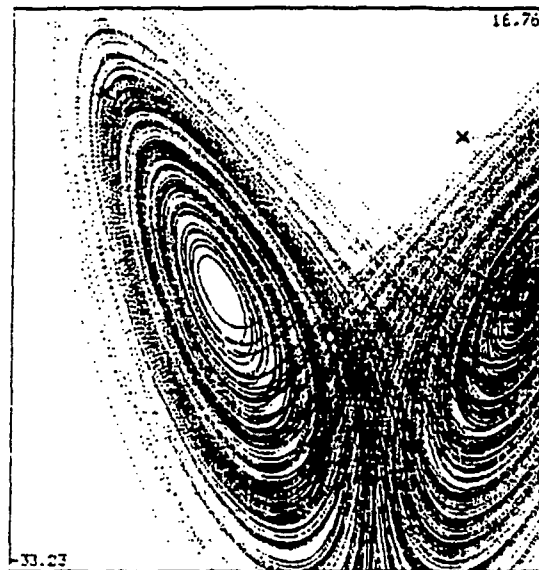
Figure 10: Without Target Acquisition
