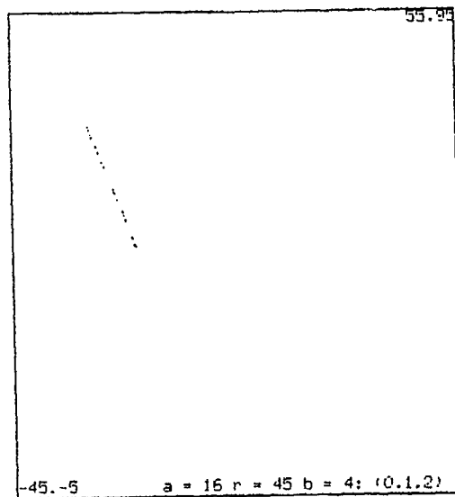
Figure 2: x-z Section of Lorenz Attractor for a = 16 , r = 45 and b = 4
