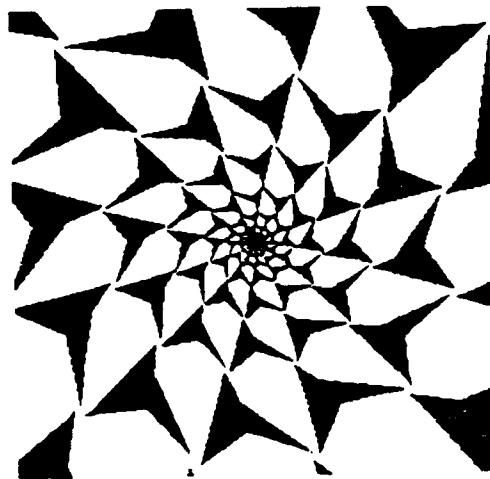
Figure 6: Iteratively applying a rotate-and-scale map to a polygon.
