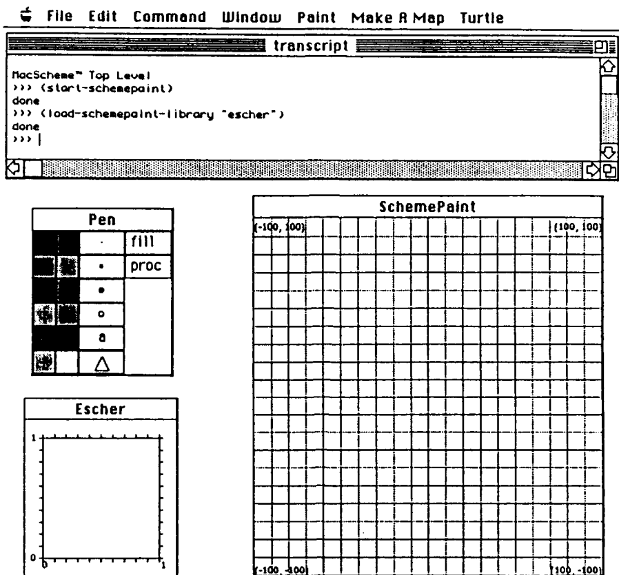
Figure 9: The SchemePaint screen, now including an "Escher palette" window.
