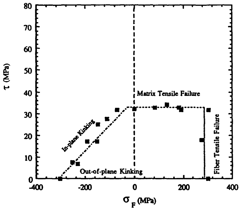
Damage Modes for Axial Loading and Torsion
