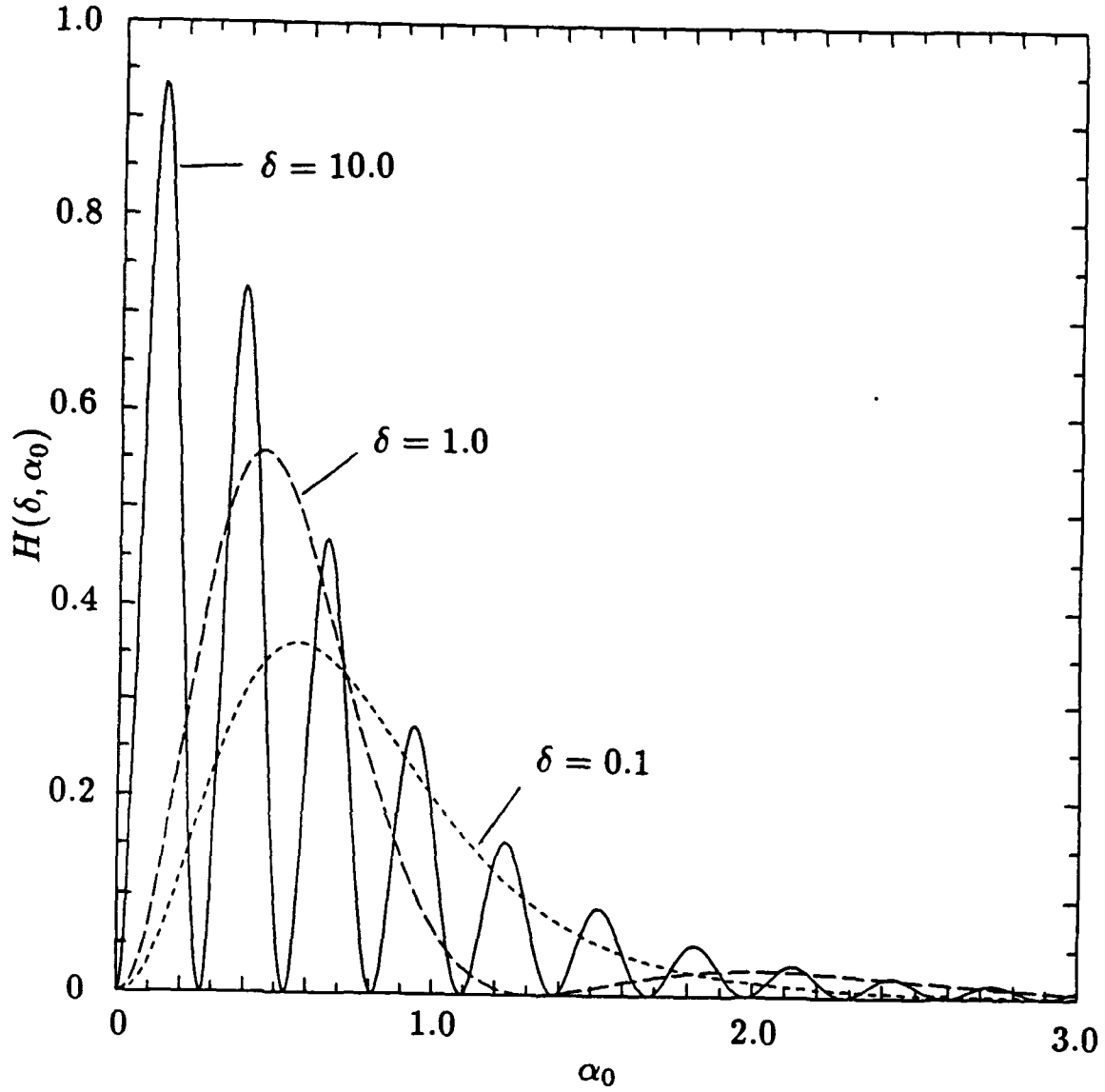
Fig. 3: The function H(\delta, \alpha_0) , proportional to the third harmonic power emerging from a plasma of width 2z_0 centered about the laser focus, verses \alpha_0 = z_0/Z_R , for \delta = 2k_p^2 r_0^2/3 = 10.0 (solid curve), 1.0 (dashed curve) and 0.1 (dotted curve), where Z_R = k_0 r_0^2/2 is the Rayleigh length.
