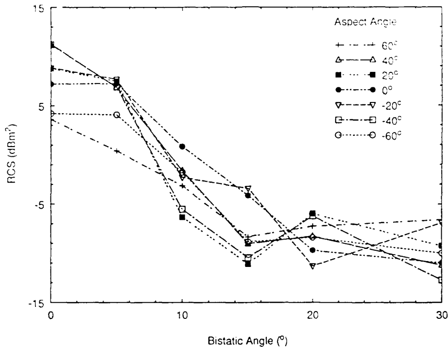
Figure 4. A plot of the average RCS for the TRX-11 over a 20 degree arc centred on the given aspect angles against increasing bistatic angle.
