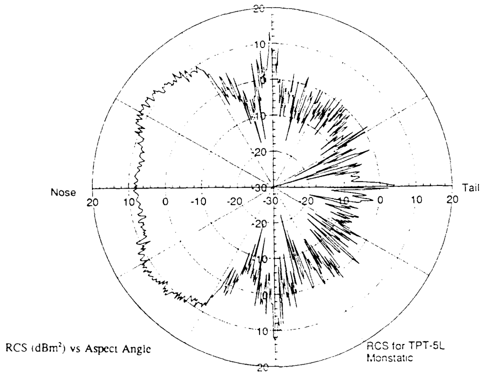
Figure 5. The RCS for the TPT-5L for the monostatic case. (Azimuth plot with roll angle zero)
