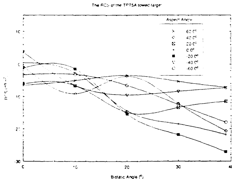
Figure 7. Cubic Spline fit of RCS data extrapolated to 39 degrees.
