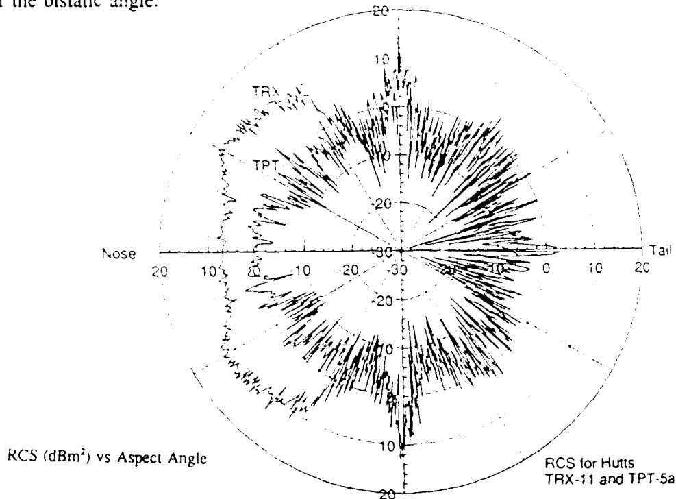
Figure 2. The RCS of the TRX-11 and TPT-5A for the monostatic case. (Azimuth plot with roll angle zero)
