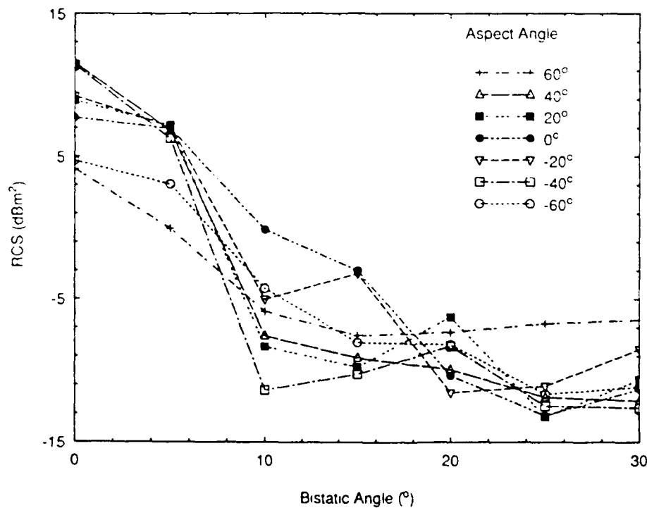
Figure 6. A plot of the average RCS for the TPT-5L over a 20 degree arc centred on the given aspect angles against increasing bistatic angle.
