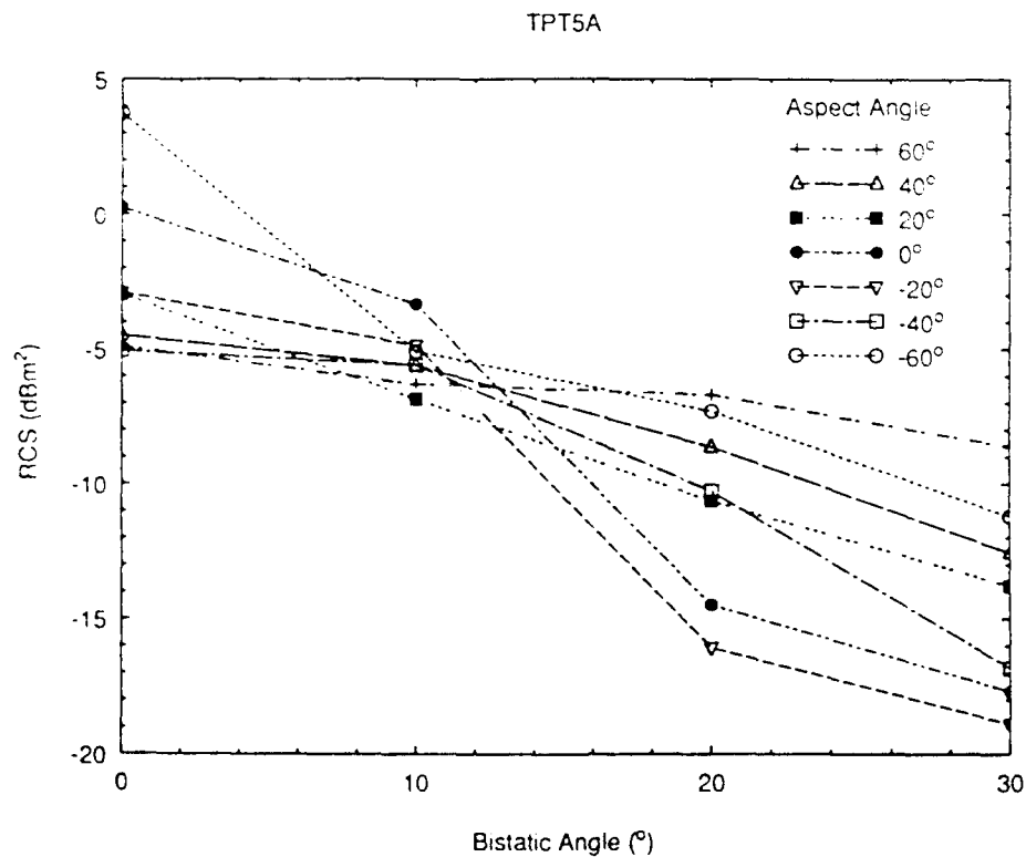
Figure 3. A plot of the average RCS for the TPT-5A over a 20 degree arc centred on the given aspect angles against increasing bistatic angle.
