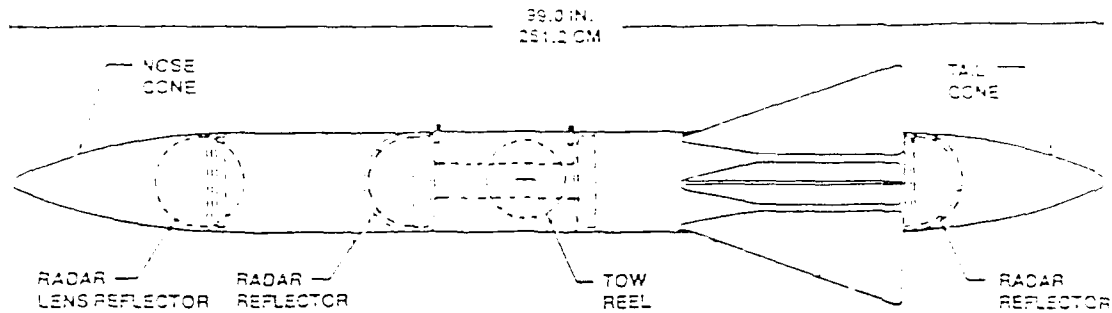
Figure 1. Outline of TRX-11 radar enhanced target.
