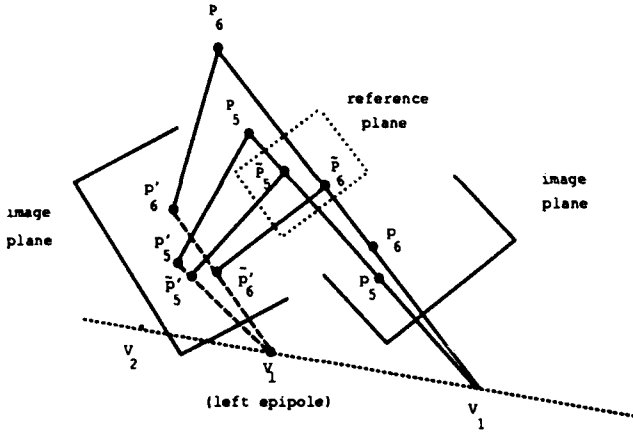
Figure 4: The geometry of locating the left epipole using two points out of the reference plane.
