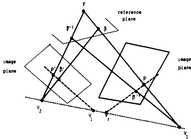
Figure 14: Epipolar lines are perspectively related.
