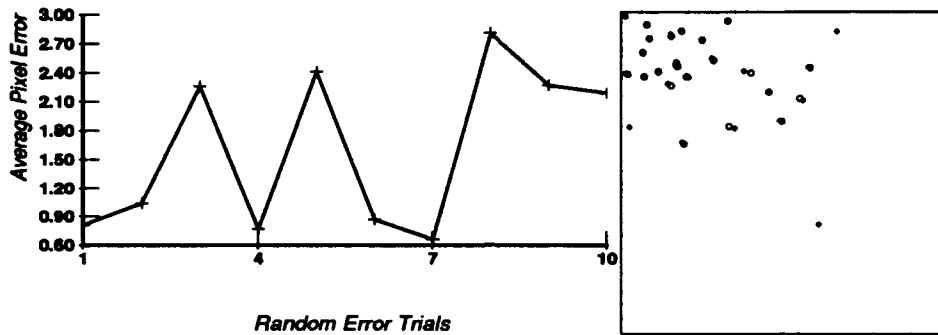
Figure 9: Random noise added to all image points, over all views, for 10 trials. Average pixel error fluctuates around 1.6 pixels. The result of re-projection on a typical trial with average error of 1.05 pixels, and maximal error of 5.41 pixels.
