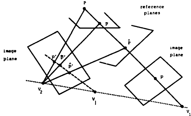
Figure 3: Definition of projective shape as the cross ratio of p', \tilde{p}', \hat{p}', V_1 .
