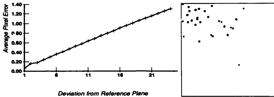
Figure 8: Deviation from coplanarity: average pixel error due to translation of P_1 along the optical axis from z = 100 to z = 125 , by increments of one unit. The result of re-projection (overlay of re-projected image and novel image) for the case z = 125 . The average error is 1.31 and the maximal error is 7.1.
