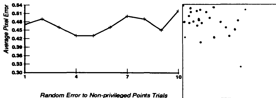
Figure 10: Random noise added to non-privileged image points, over all views, for 10 trials. Average pixel error fluctuates around 0.5 pixels. The result of re-projection on a typical trial with average error of 0.52 pixels, and maximal error of 1.61 pixels.
