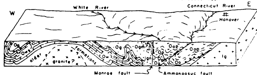
Figure 13. Idealized geologic history of the Upper Valley area (from Lyons 1958).
