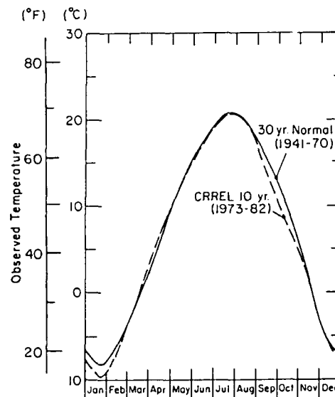
Figure 23. Temperature data from CRREL (dashed line) and Hanover, New Hampshire (after Bates 1984).
