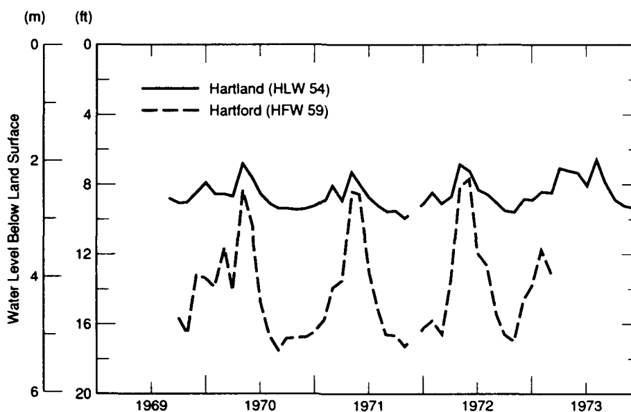
Figure 25. Seasonal fluctuation of water levels in two wells in the White River Junction area (after Hodges et al. 1976).
