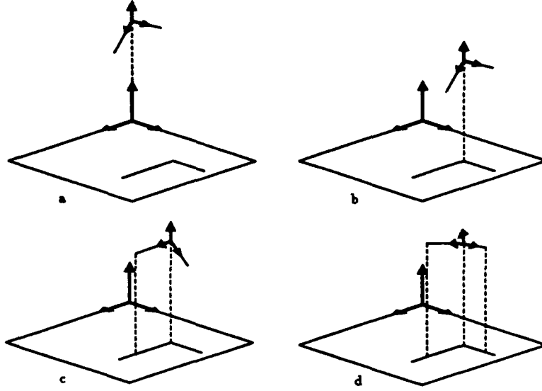
Figure 1: Computing the pose. Part a: A pair of basis vectors in the image have been selected, as well as a pair of model basis vectors. The origin of the model basis is assumed to project to the origin of the image coordinate system. Part b: After the translation, the origin point of the selected model basis projects to the origin of the selected image basis. Part c: After the first rotation, the first model axis projects along the first image axis. Part d: After the next two rotations, both model axes project along their corresponding image axis, such that the ratios of the lengths of the axes are the same in the projected model and the image.
