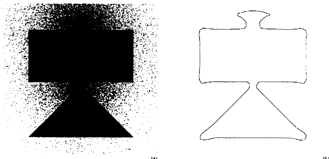
Figure 13: Zero-crossings of the Laplacian of Gaussian filter. Ideally, the zero-crossings of the Laplacian of Gaussian filter demark discontinuities in the brightness of the image. However, it is well known that in areas of low contrast, the zero-crossings often wander away from the subjective location of the discontinuity. Furthermore, nearby regions tend to interfere with one another such that the subjective regions blend together. A synthetic image of a rectangle and a triangle on a textured background is shown in (a). The zero-crossings of a Laplacian of Gaussian filter illustrate the undesired effects in (b). Notice that the zero-crossings wander away from the rectangle at the top and the triangle blends together with the rectangle.
