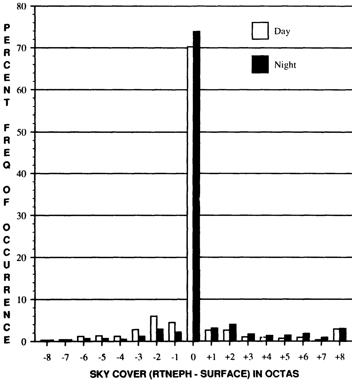
Figure 14. Comparison of Day/Night RTNEPH minus Surface Observations, mid-Latitudes, Summer.
