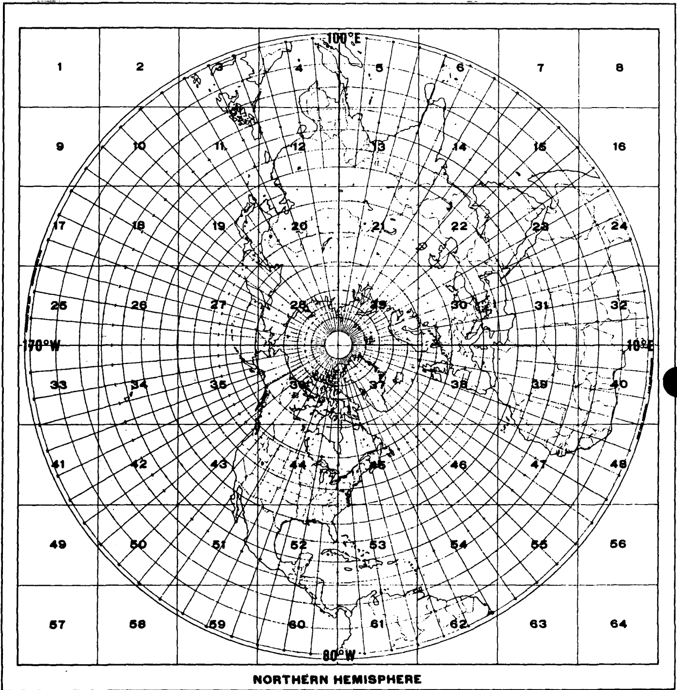
Figure 1. Northern Hemisphere RTNEPH grid over a polar-stereographic projection. Corner boxes are not used.
