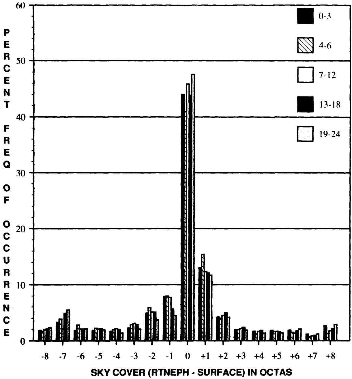
Figure 27. Comparison of RTNEPH and Surface Report Differences for Different Time-Lag Hour Groups, All Latitudes, Autumn.
