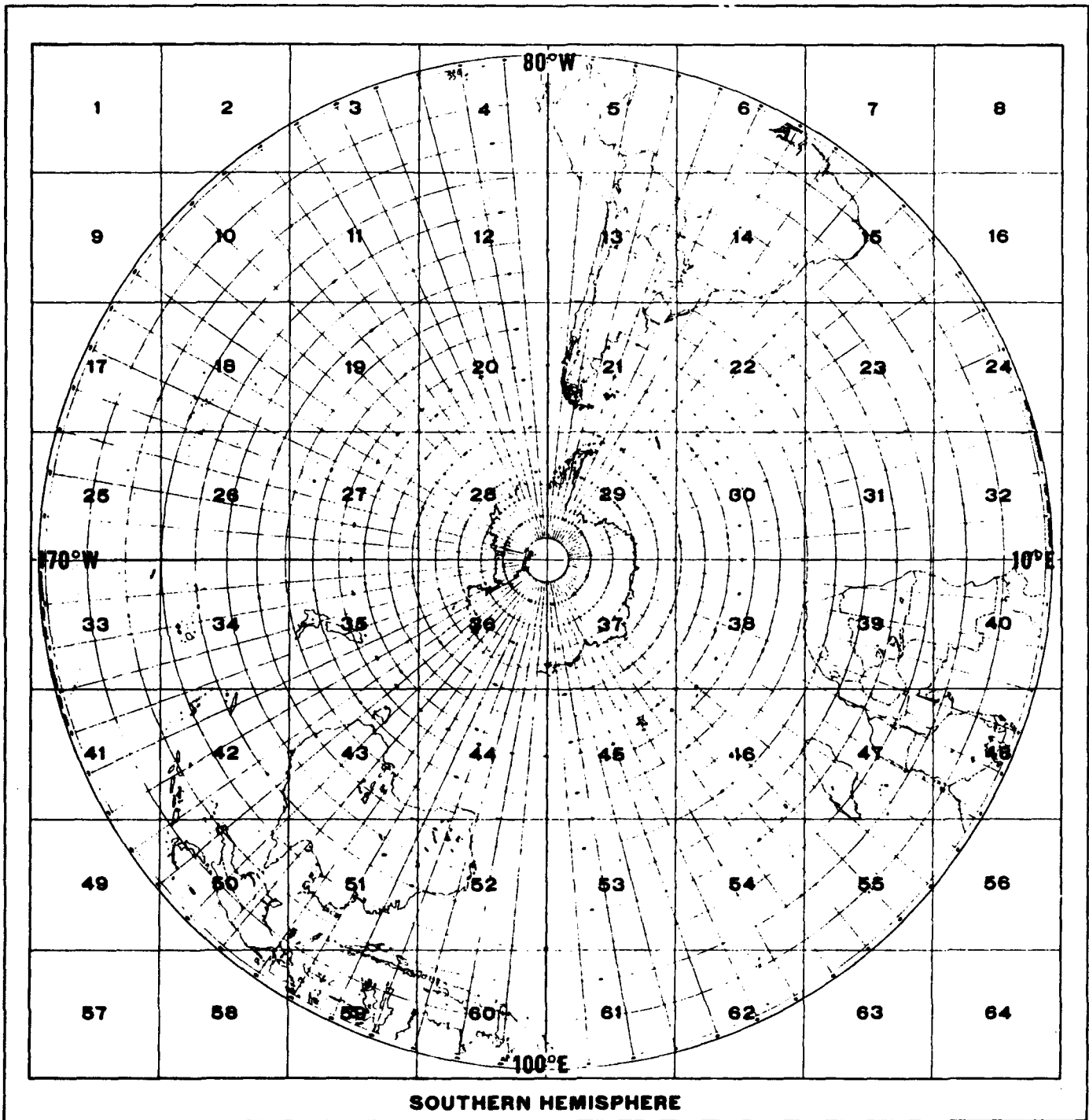
Figure 2. Southern Hemisphere RTNEPH grid over a polar-stereographic projection. Corner boxes are not used. Add 100 to the box numbers shown.
