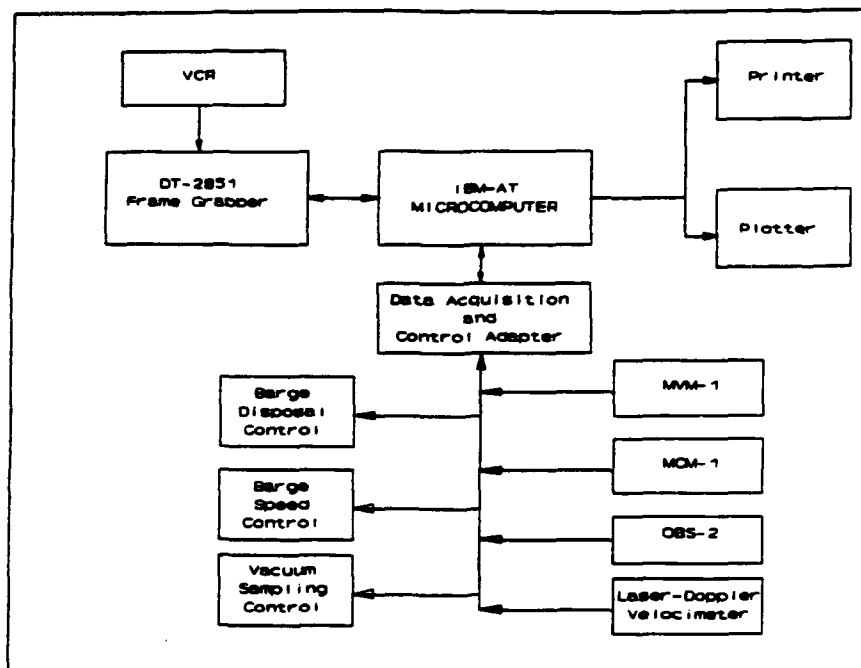
Figure 8. Microcomputer-based data management system
