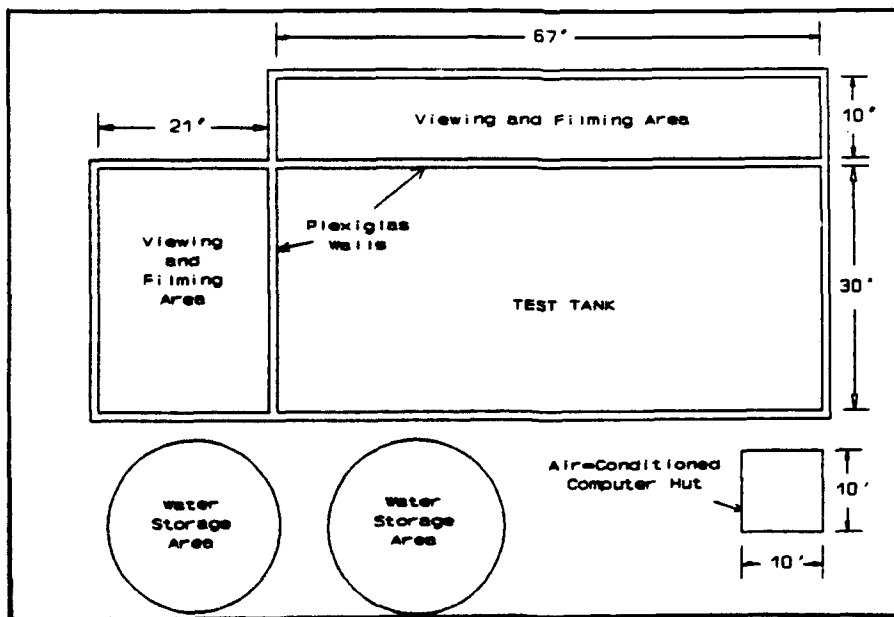
Figure 7. Georgetown Harbor sump, alternative design 3
