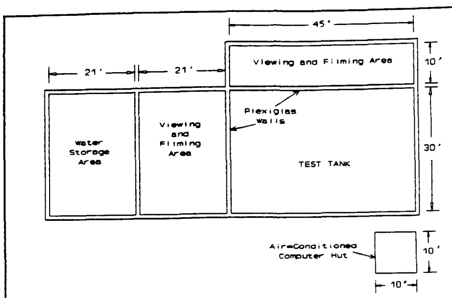
Figure 6. Georgetown Harbor sump, alternative design 2
