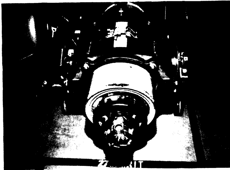
Figure 18a. Sperry 200 KeV X-Ray Unit
