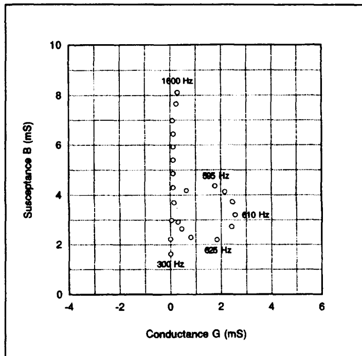
Figure 15 Admittance circle.
