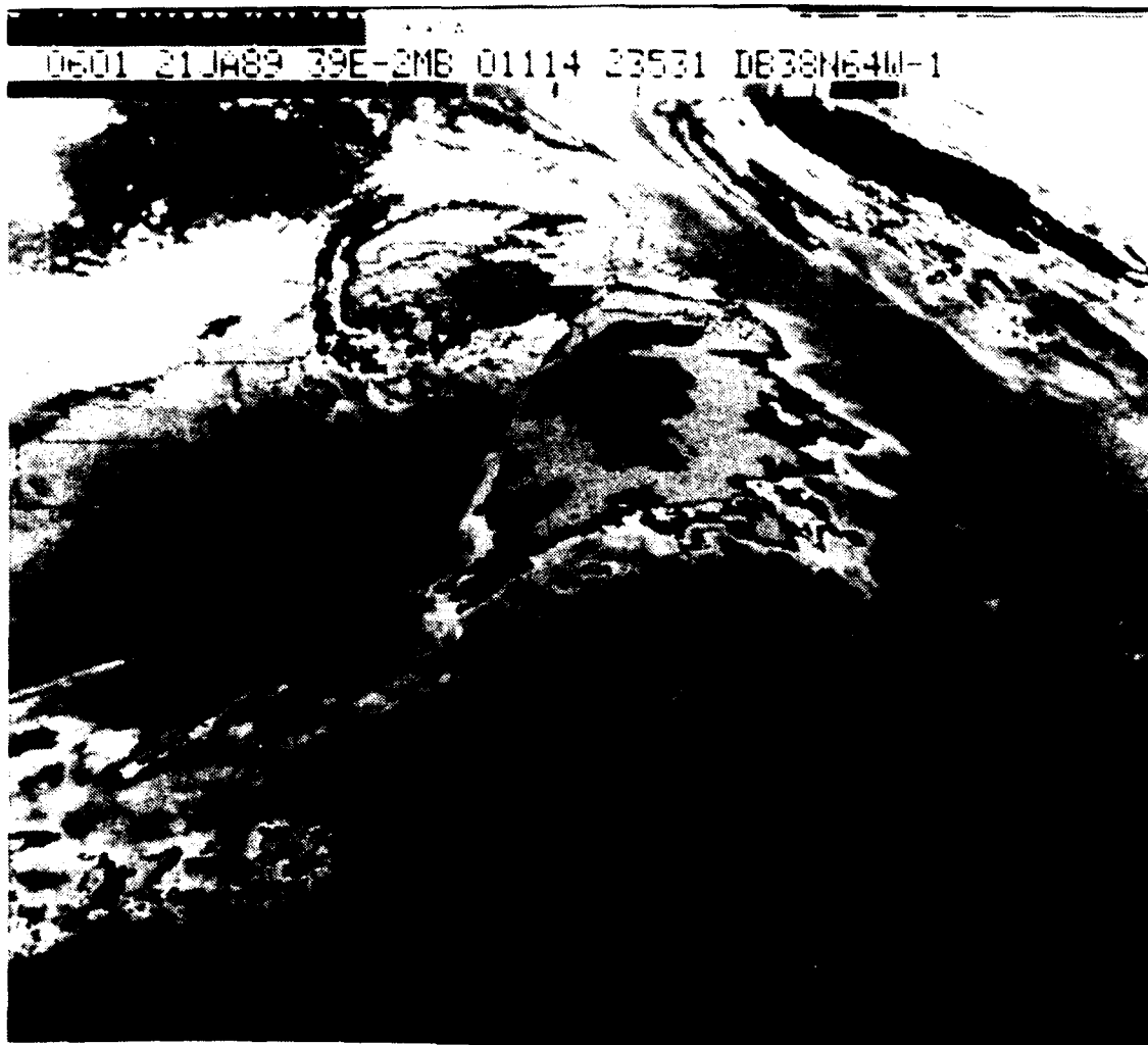
Figure 20. GOES enhanced IR imagery at 0601 UTC 21 January 1989.
