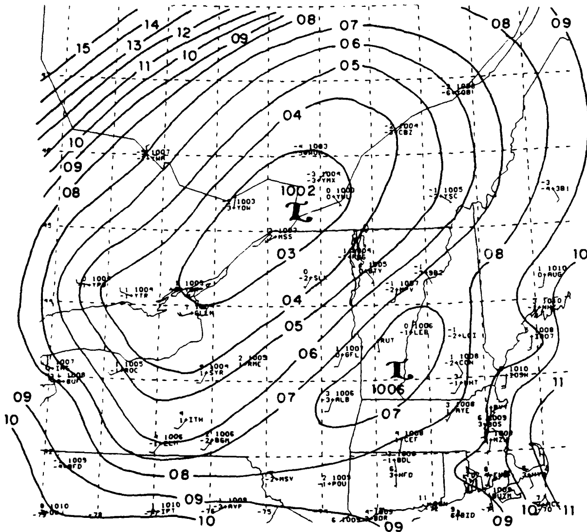
Figure 38. Subjective surface pressure (solid, contour interval 1 mb) analysis at 1500 UTC 20 January 1989.
