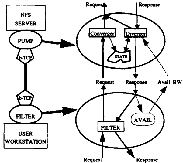
Figure 12: The filter and pump mechanisms
