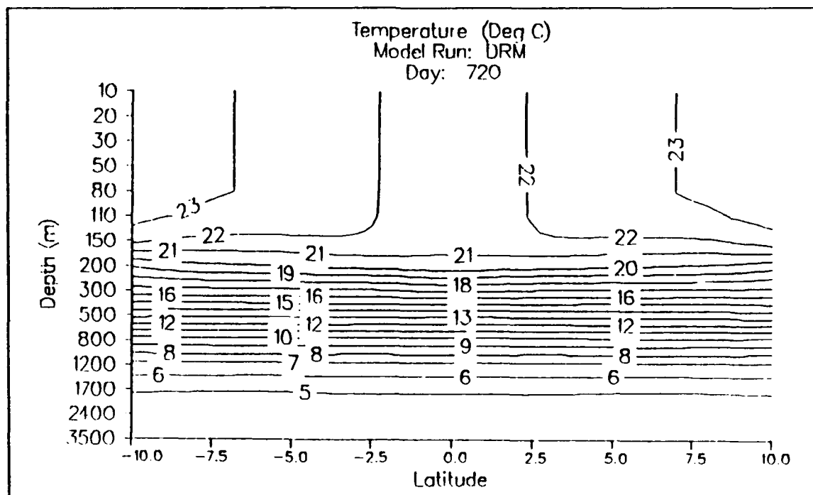
Figure 3.17. Development run DRM temperature y-z cross section through mid-basin. Contour interval is 1.0°C.
