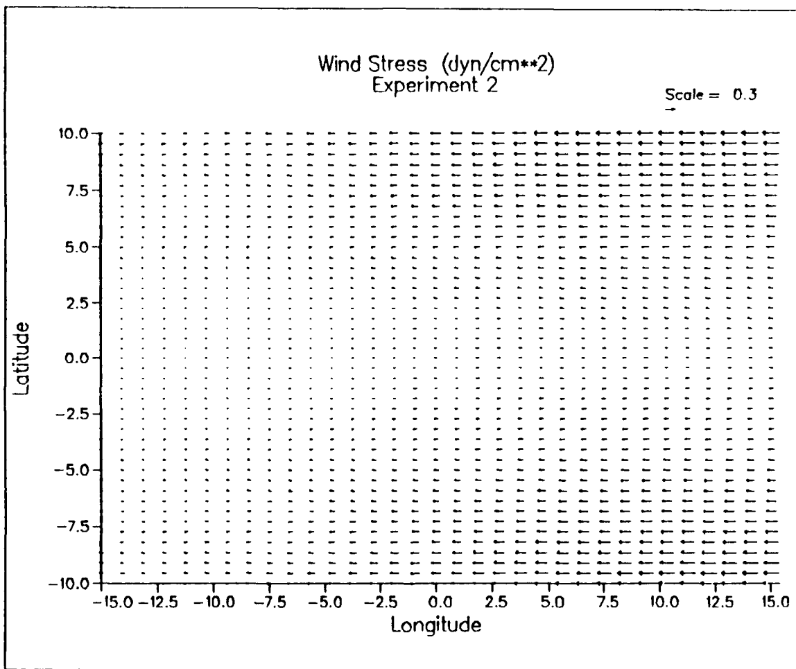
Figure 3.45. Experiment 2 wind stress: zonal component varies zonally and meridionally; no meridional component.
