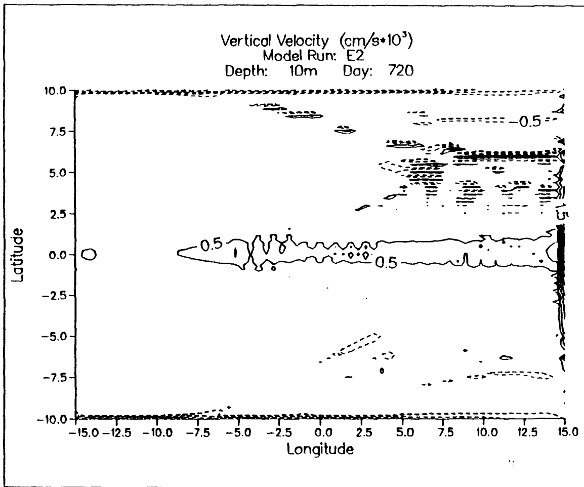
Figure 3.60. Experiment 2 10 m vertical velocity. Contour interval is 0.5 \times 10^3 \text{ cm/s} . Solid lines depict positive values; dashed lines depict negative values.
