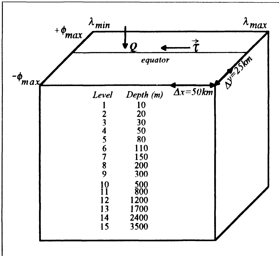
Figure 2.1. Model domain schematic:
