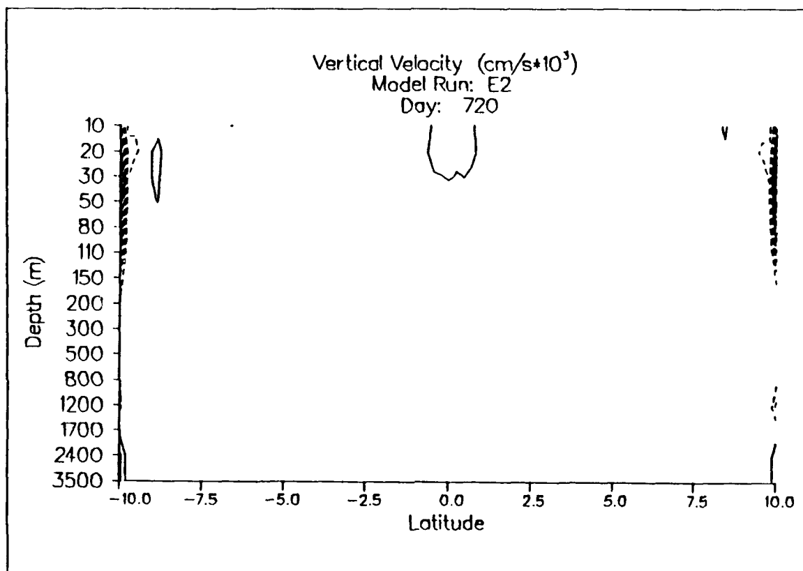
Figure 3.61. Experiment 2 vertical velocity y-z cross section through mid-basin. Contour interval is 0.5 \times 10^3 \text{ cm/s} . Solid lines depict positive values; dashed lines depict negative values.
