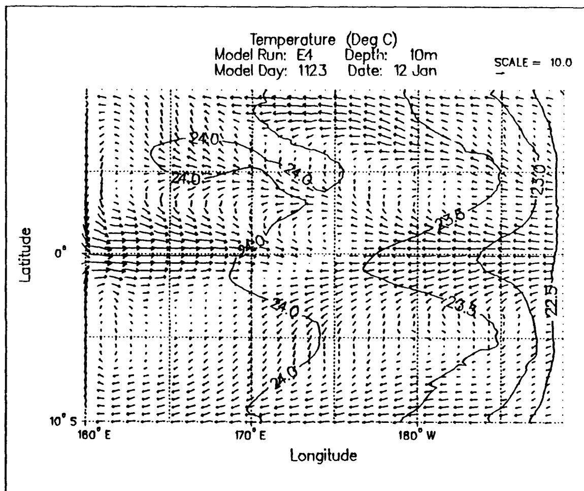
Figure 3.78. Experiment 4 10 m temperature and horizontal currents (cm/s) for model day 1123: Note the cold protrusion along approximately 5°N and the strengthening of the SEC extending from the eastern boundary. Contour interval is 0.5°C.
