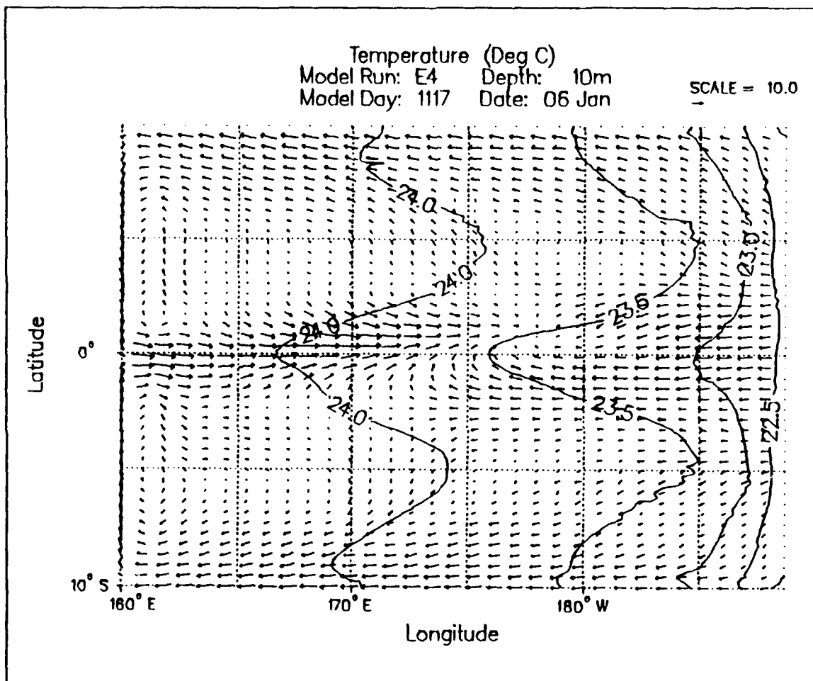
Figure 3.76. Experiment 4 10 m temperature and horizontal currents (cm/s) for model day 1117: Note the diminished reversal of the SEC in the western basin. Contour interval is 0.5^{\circ}\text{C} .
