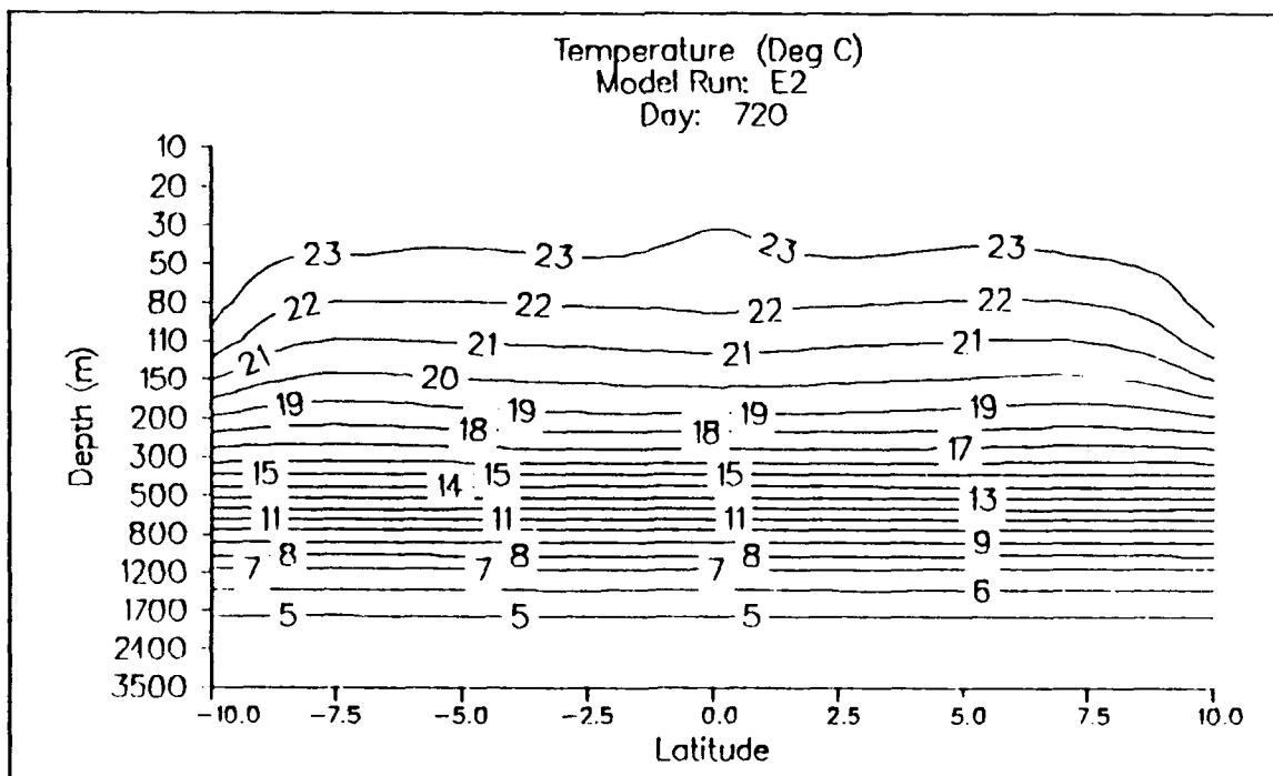
Figure 3.59. Experiment 2 temperature y-z cross section through mid-basin. Contour interval is 1.0°C.
