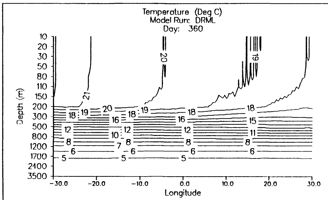
Figure 3.39. Development run DRML temperature x-z cross section along the equator. Contour interval is 1.0°C.
