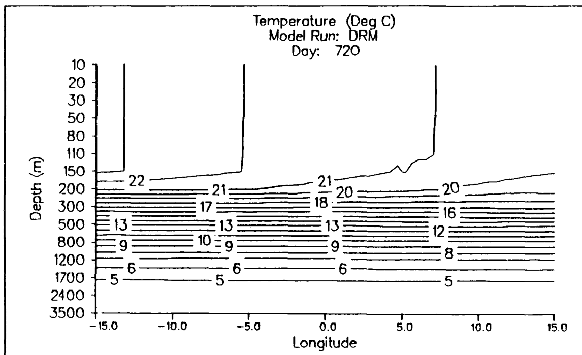
Figure 3.16. Development run DRM temperature x-z cross section along the equator. Contour interval is 1.0°C.
