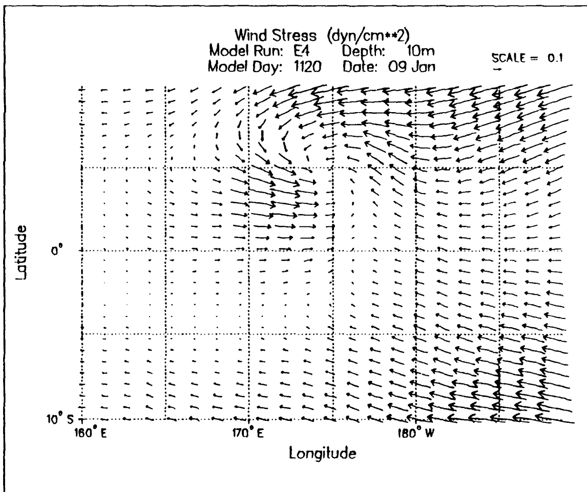
Figure 3.73. Experiment 4 wind stress (dyns/cm 2 ) for model day 1120: Note the westerly wind event in the mid-basin associated with Typhoon Axel.
