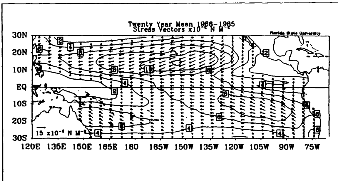
Figure 4.4. Mean wind stress vectors for the tropical Pacific after Stricherz et al. (1992).
