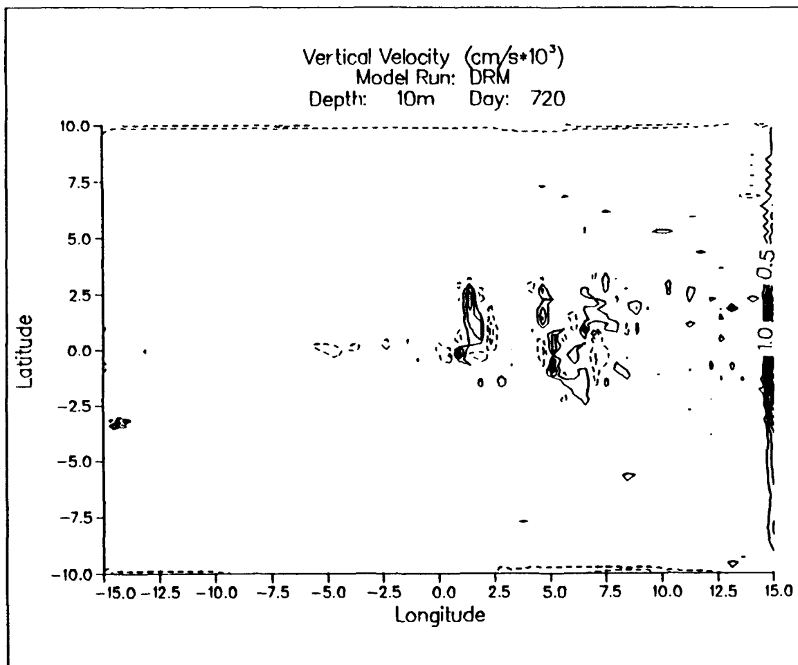
Figure 3.18. Development run DRM 10 m vertical velocity. Contour interval is 0.5 \times 10^3 \text{ cm/s} . Solid lines depict positive values; dashed lines depict negative values.
