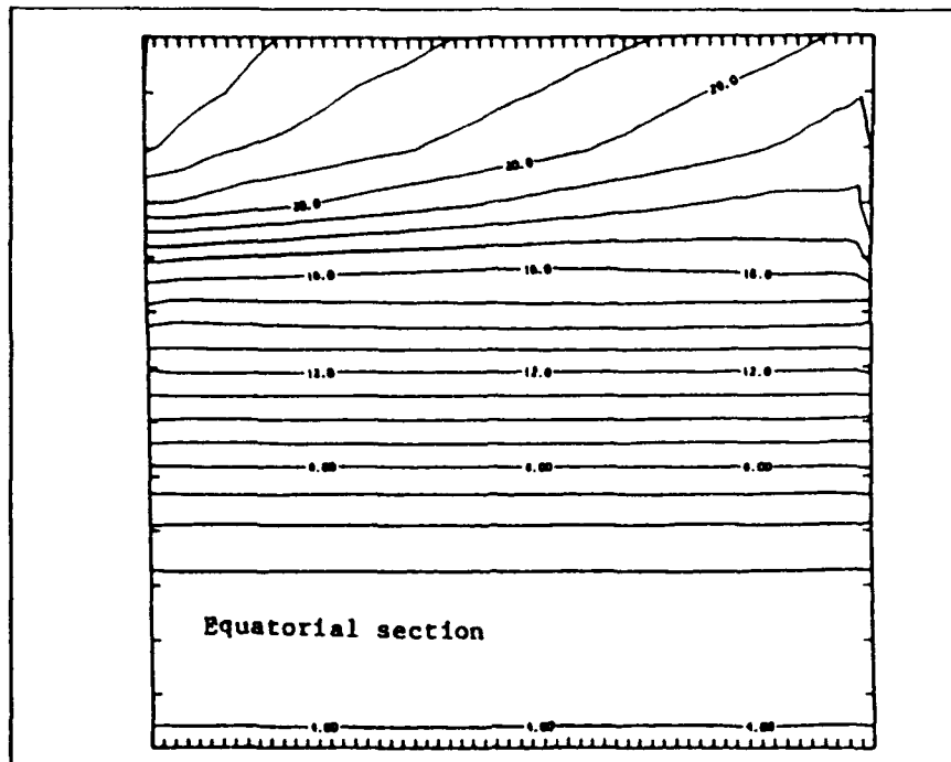
Figure 4.2a. Zonal temperature profile along the equator after Semtner and Holland (1980).
