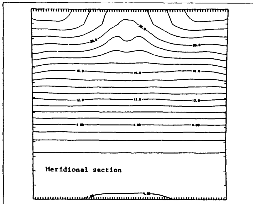
Figure 4.2b. Meridional temperature profile after Semtner and Holland (1980).
