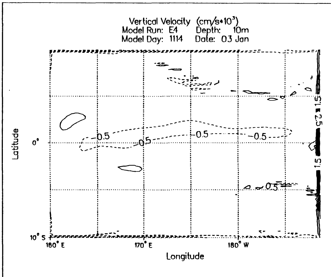
Figure 3.79. Experiment 4 10 m vertical velocity for model day 1114: Note the downwelling area along the equator. Contour interval is 0.5 \times 10^3 \text{ cm/s} .
