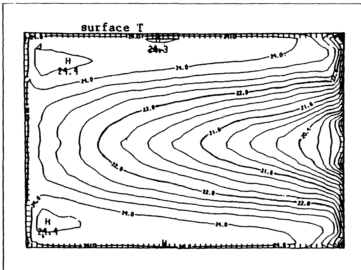
Figure 4.1. Surface temperature contours after Semtner and Holland (1980).
