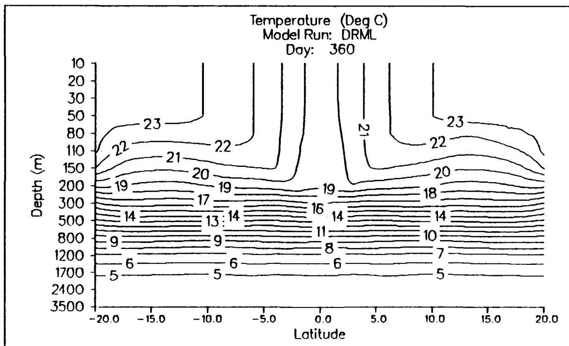
Figure 3.40. Development run DRML temperature y-z cross section through mid-basin. Contour interval is 1.0°C.
