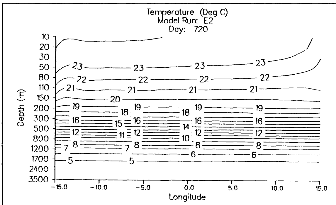
Figure 3.58. Experiment 2 temperature x-z cross section along the equator. Contour interval is 1.0°C.
