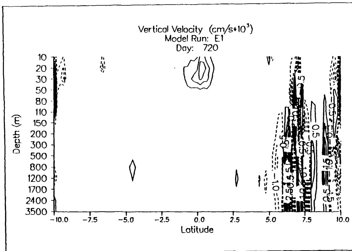
Figure 3.53. Experiment 1 vertical velocity y-z cross section through mid-basin. Contour interval is 0.5 \times 10^3 cm/s. Solid lines depict positive values; dashed lines depict negative values.
