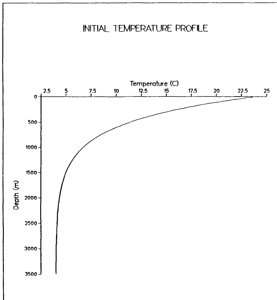
Figure 2.3. Initial temperature profile.
