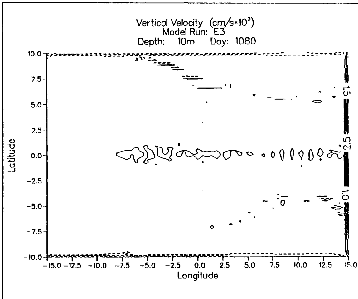
Figure 3.68. Experiment 3 10 m vertical velocity. Contour interval is 0.5 \times 10^3 cm/s. Solid lines depict positive values; dashed lines depict negative values.
