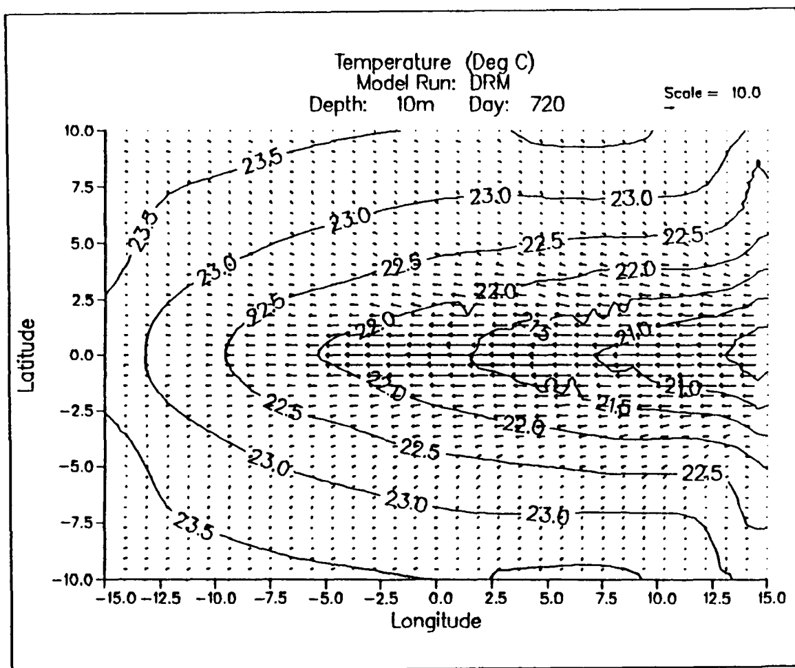
Figure 3.13. Development run DRM 10 m temperature and horizontal currents (cm/s). Contour interval is 0.5°C.
