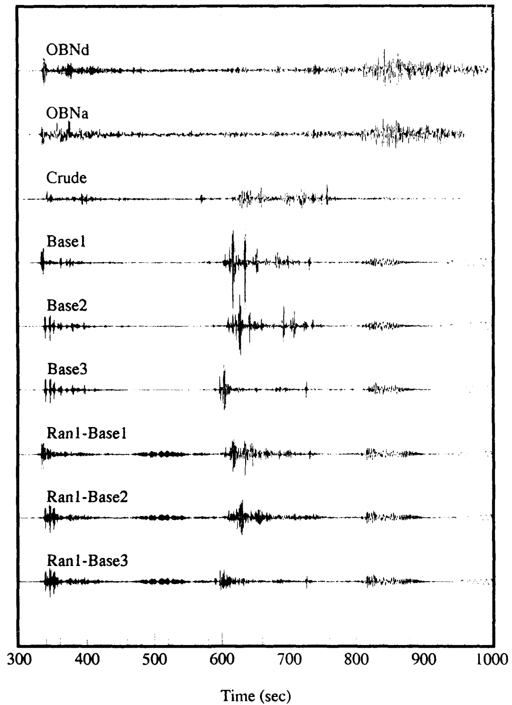
Figure 14. Comparisons of data with synthetic seismograms at OBN. The data station names end in "d" to signify the digital data or "a" to signify the analog data.
