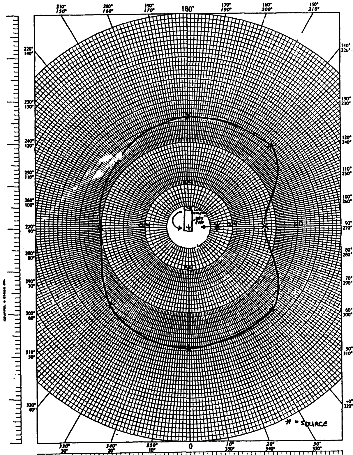
Figure 11. Angular response of end window ADM-300 rotated around the x-axis.
