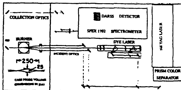
Fig. 2 Arrangement of the CARS System Optics
