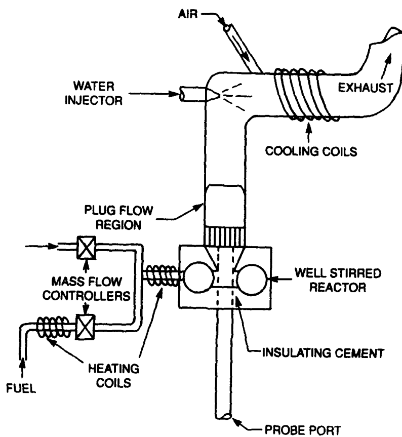
Figure 10. Schematic diagram of a PSR test facility setup
