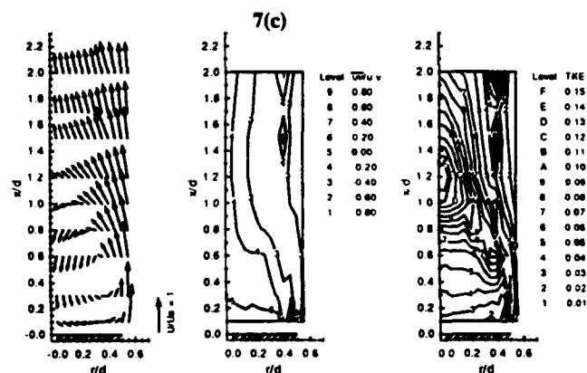
Fig. 7 Mean flow structure, Reynolds shear stresses, and turbulent kinetic energy plotted to illustrate the effects of approach turbulence intensity on turbulence flowfield. All measurements, except (c) below, are in a confined combustor flow (BR = 25%, \theta = 45 degrees, \phi = 0.65 , U = 15 m/s): (a) approach turbulence intensity, I = 22\% , (b) approach turbulence intensity, I = 17\% , (c) confined cold flow, I = 17\% .
