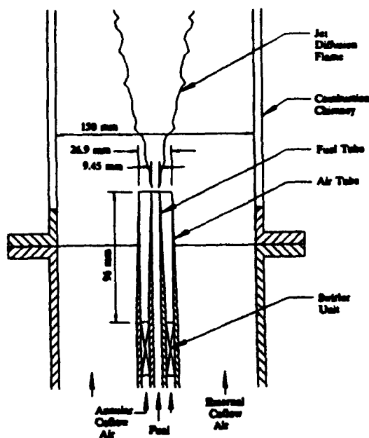
Fig. 1 Burner system configuration.
