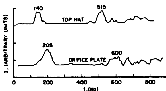
Fig. 9: Acoustic characteristics of top-hat and orifice plate outlet restrictions of same blockage ratio ( B = 0.45 ) for combustor configuration III ( \dot{v}_a = 1500 LPM, \dot{v}_f = 36 LPM).
