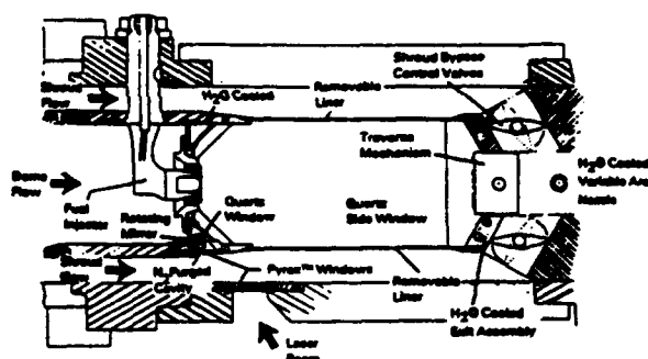
Fig. 7 Design features of generic combustor.
