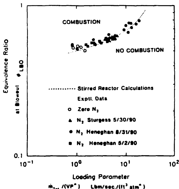
Fig. 6 Correlated blowout data for the research combustor, and comparison with the calculated well-stirred reactor blowout characteristic for the research combustor.
