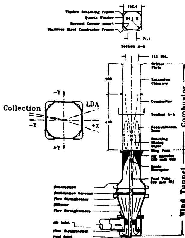
Fig. 4 Research combustor.
