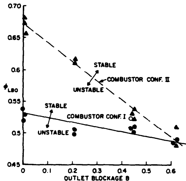
Fig. 7: Combustion stability (as measured by \phi_{LBO} vs. B) of combustor configurations I and II in the near-turbulent flow regime ( Re < 23,000 ). Note that m/VP^2 ( U - U_f/U ) = 0.8 configuration I and = 1.6 for configuration II.
