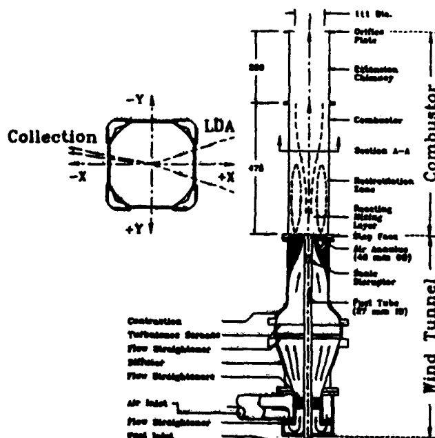
Fig. 1 Research Combustor, Showing Axis Convention
