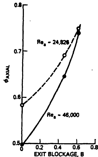
Fig. 13: Influence of orifice plate outlet blockage, B on the equivalence ratio for the onset of axial instability in the lifted flame.
