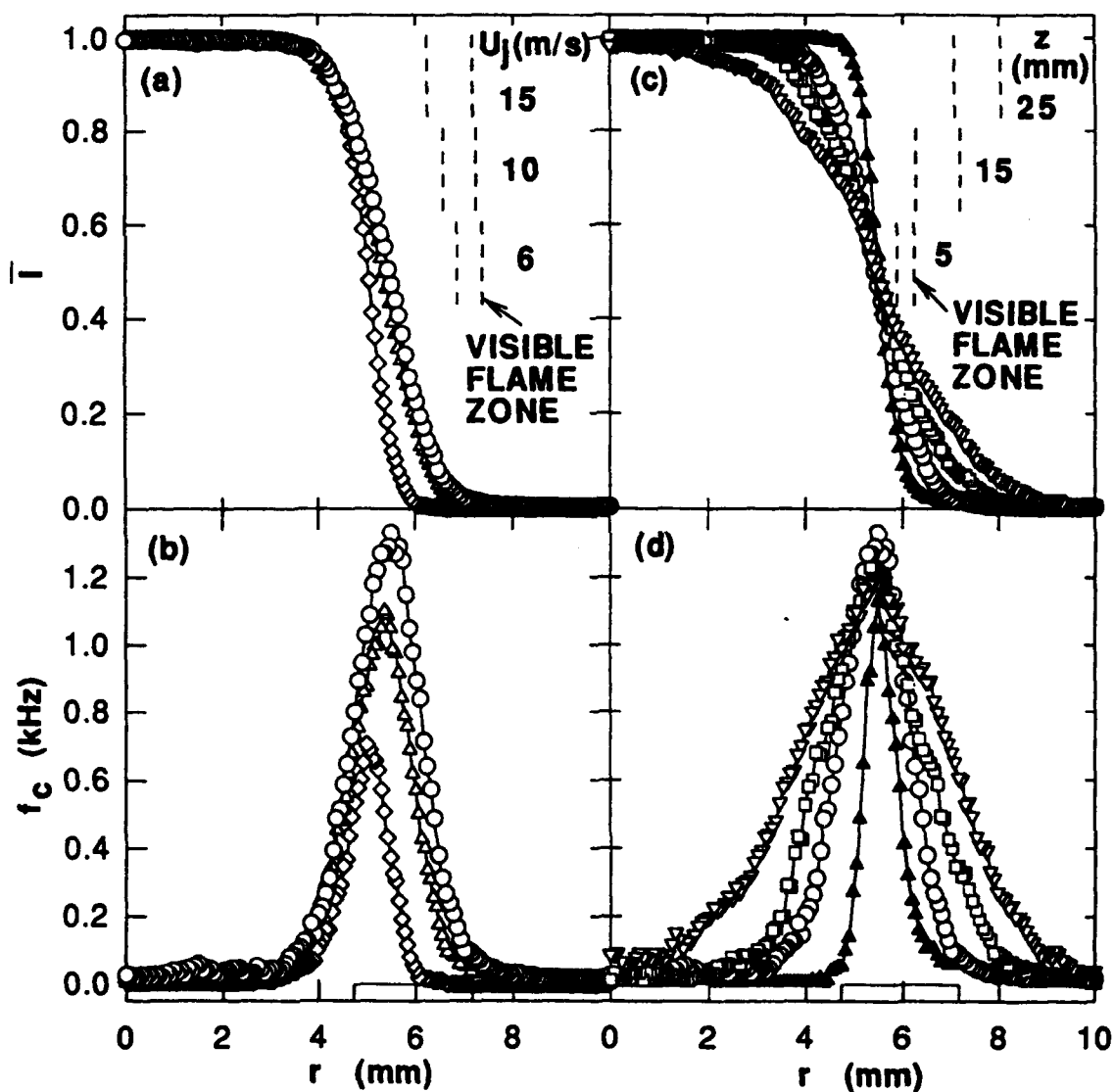
Figure 3 Radial profiles of the intermittency and crossing frequency of the jet fluid in a methane/air coflow jet diffusion flame. U_a=3 m/s. (a)(b) z=15 mm. \diamond , U_f=6 m/s; \Delta , U_f=10 m/s; \circ , U_f=15 m/s. (c)(d) U_f=15 m/s. \blacktriangle , z=5 mm; \circ , z=15 mm; \square , z=25 mm; \nabla , z=50 mm.
