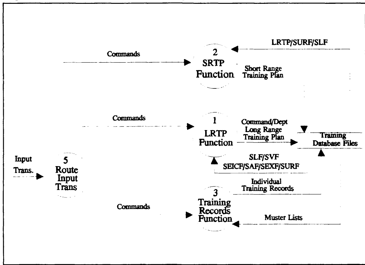
Figure 3.1 Level 1 Data Flow Diagram
