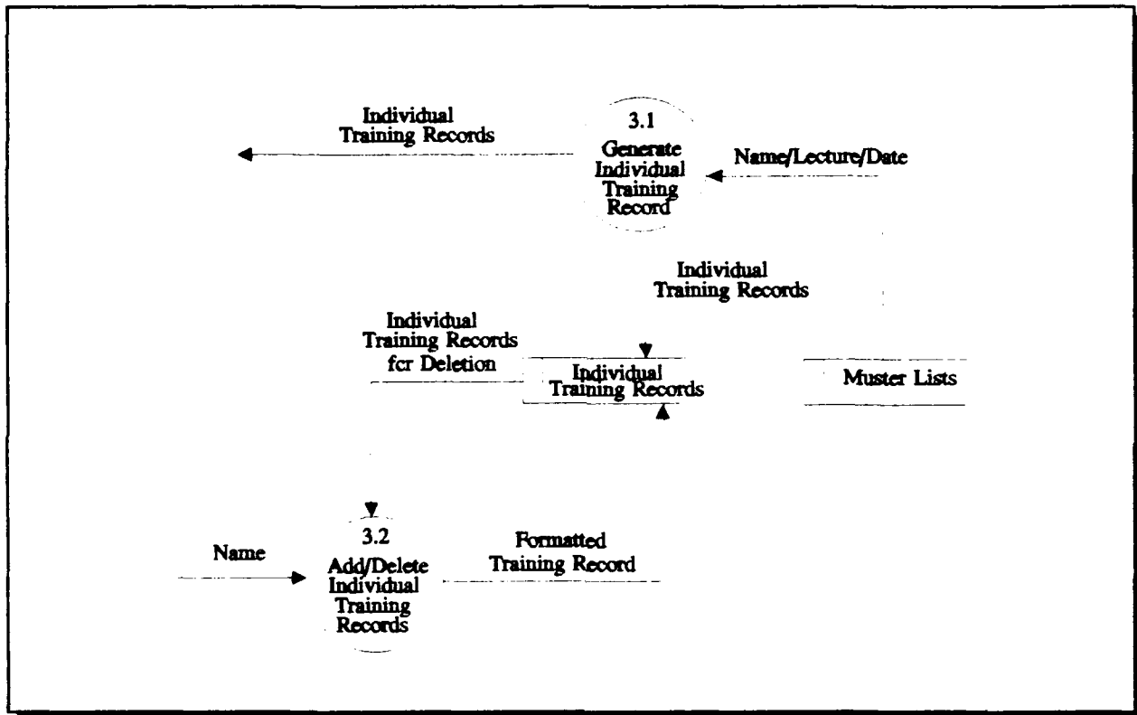
Figure 4-3: Individual Training Records DFD
