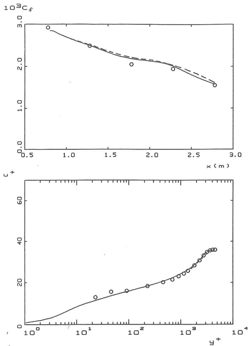
Figure 3.3: Flow 1200: Incompressible boundary layer with strong adverse pressure gradient; \circ Ludweig-Tillman; — k-\omega with viscous corrections; - - - k-\omega without viscous corrections.
